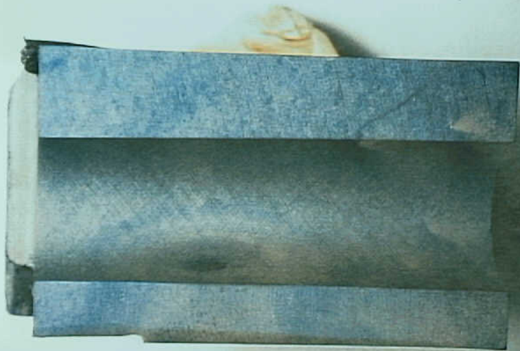
Photo 20. Hole #1B after deviding and BEA. The ID exhibit an BEA indication consisting of a mostly blue elliptic spot with surrounding area which indicated alternaterly in grey and blue. Compare with photo 16.
