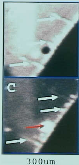
Photo 2. Oxygen and carbon SIMS maps from first region examined. White indicated higher elemental concentrations. Both oxygen and carbon were observed to be concentrated in the "hardened layer" as well as in the cracks (white arrows). A carbon-rich patch
