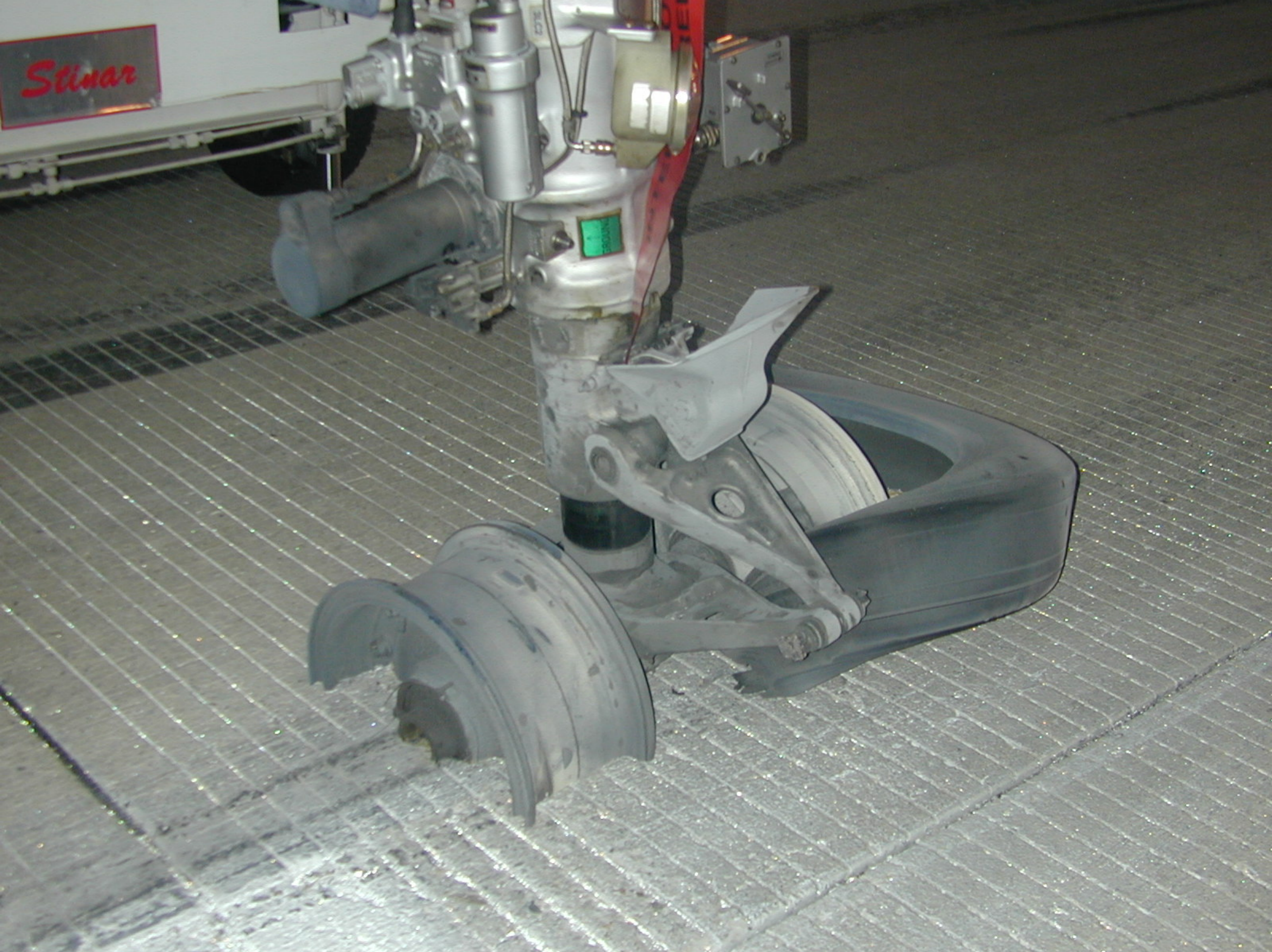
Photo 1-Nose Landing Gear on Runway
