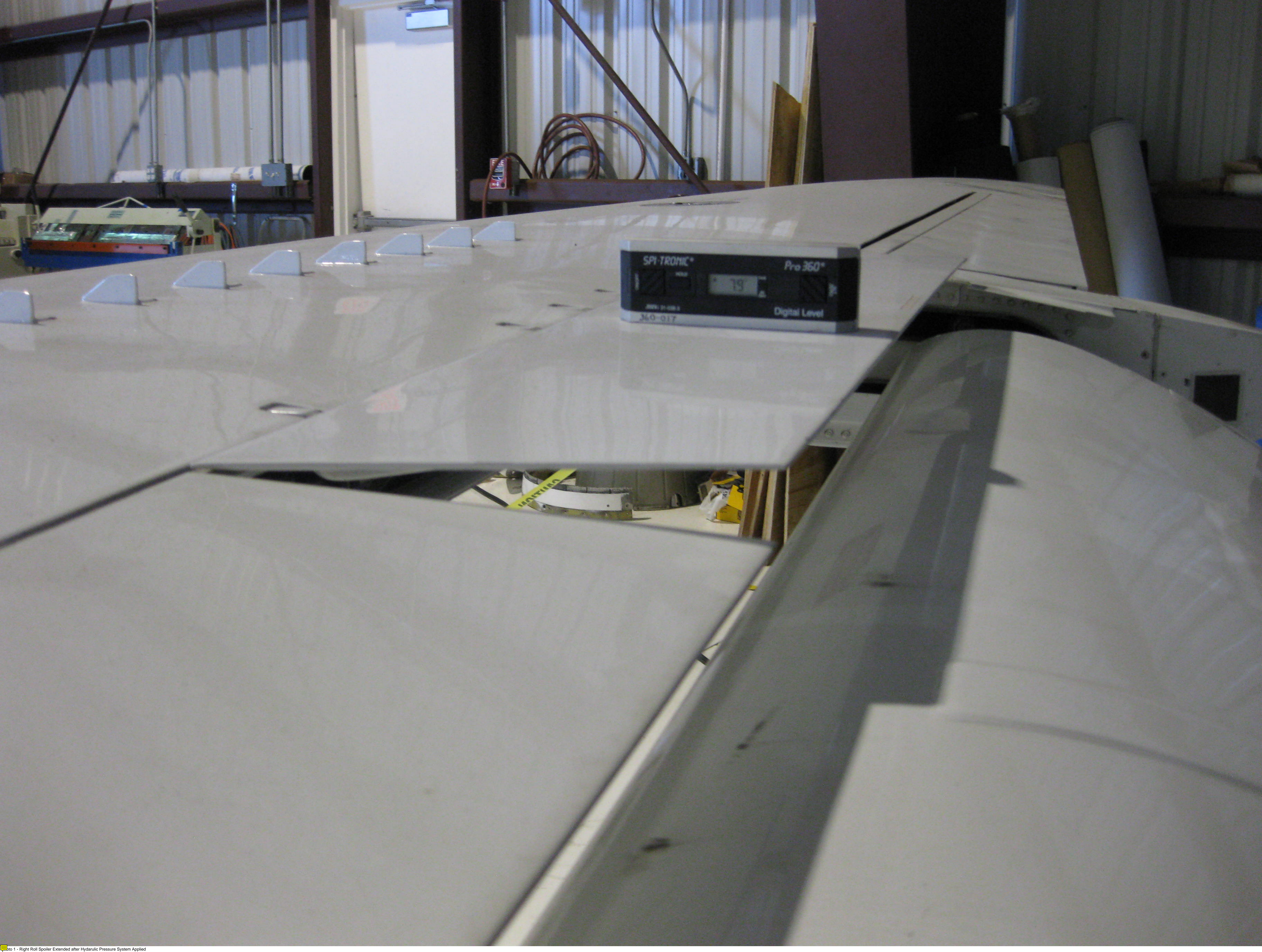
Photo 1 - Right Roll Spoiler Extended after Hydraulic Pressure System Applied
