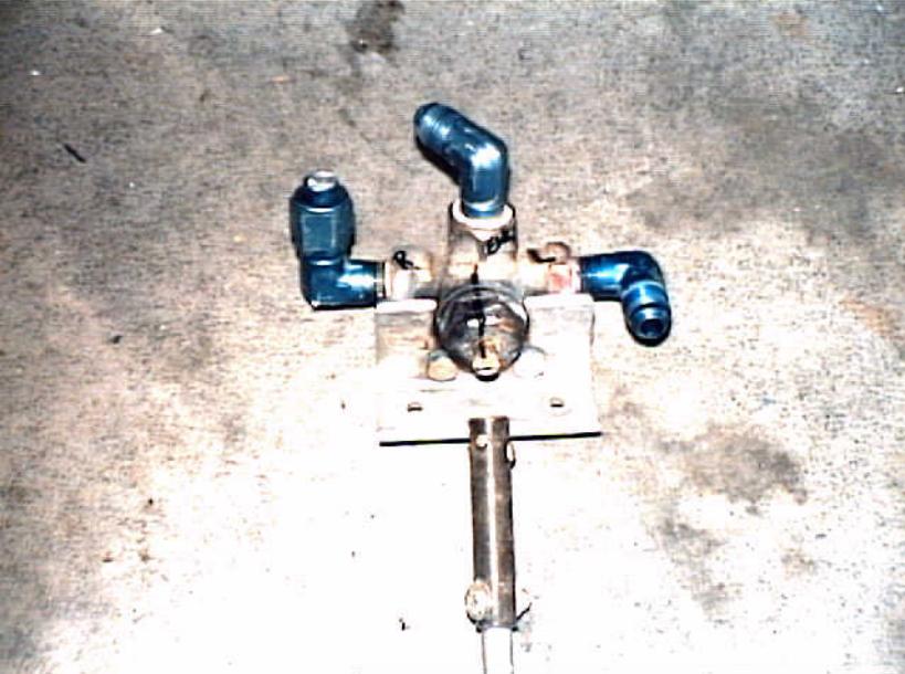
Photo 18. Fuel selector valve and torque tube end.
