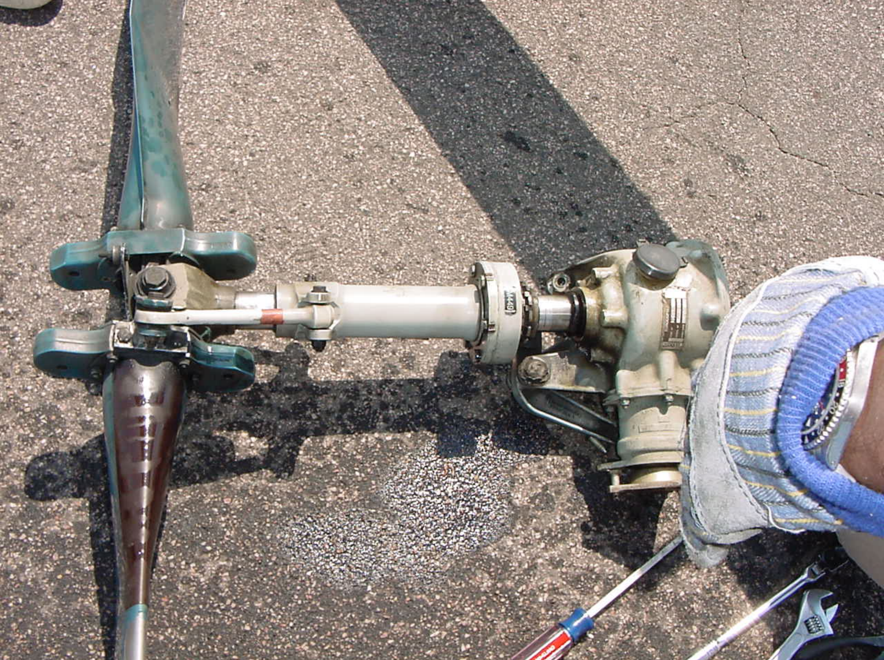
Photo 17. Tail Rotor Assembly
