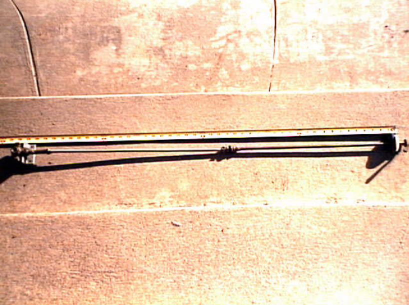
Photo 17. Distance (45") from fuel selector handle to valve.
