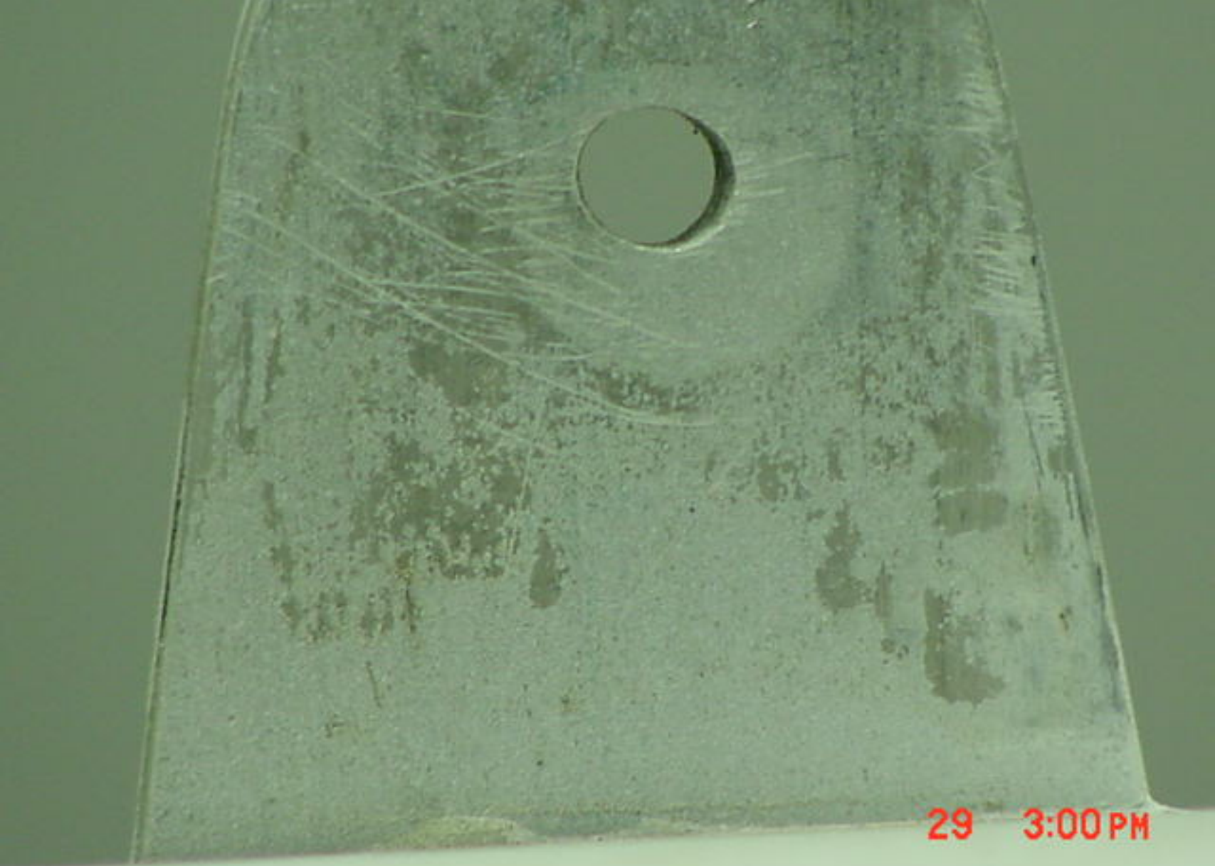
Photo 17. Canard Attachment Tab. Left Side
