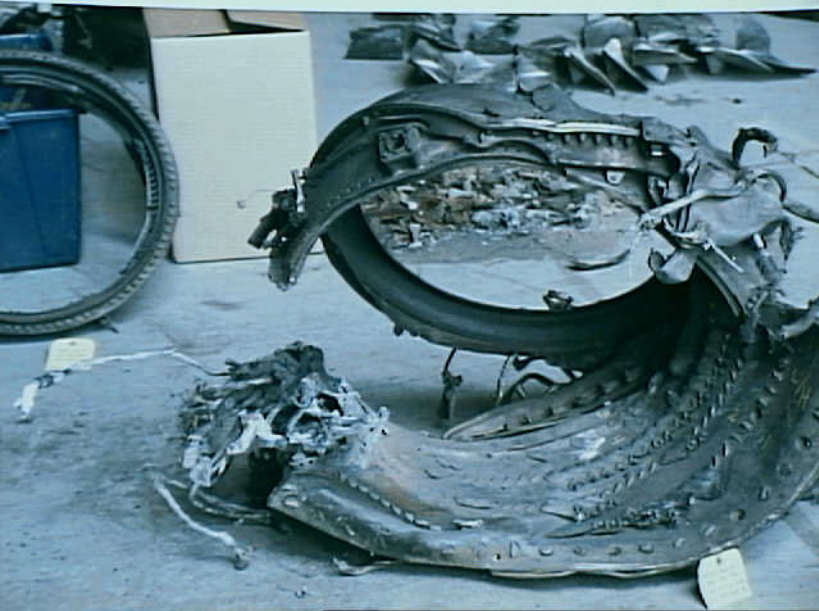
Photo 16. No. 2 engine HPC case
