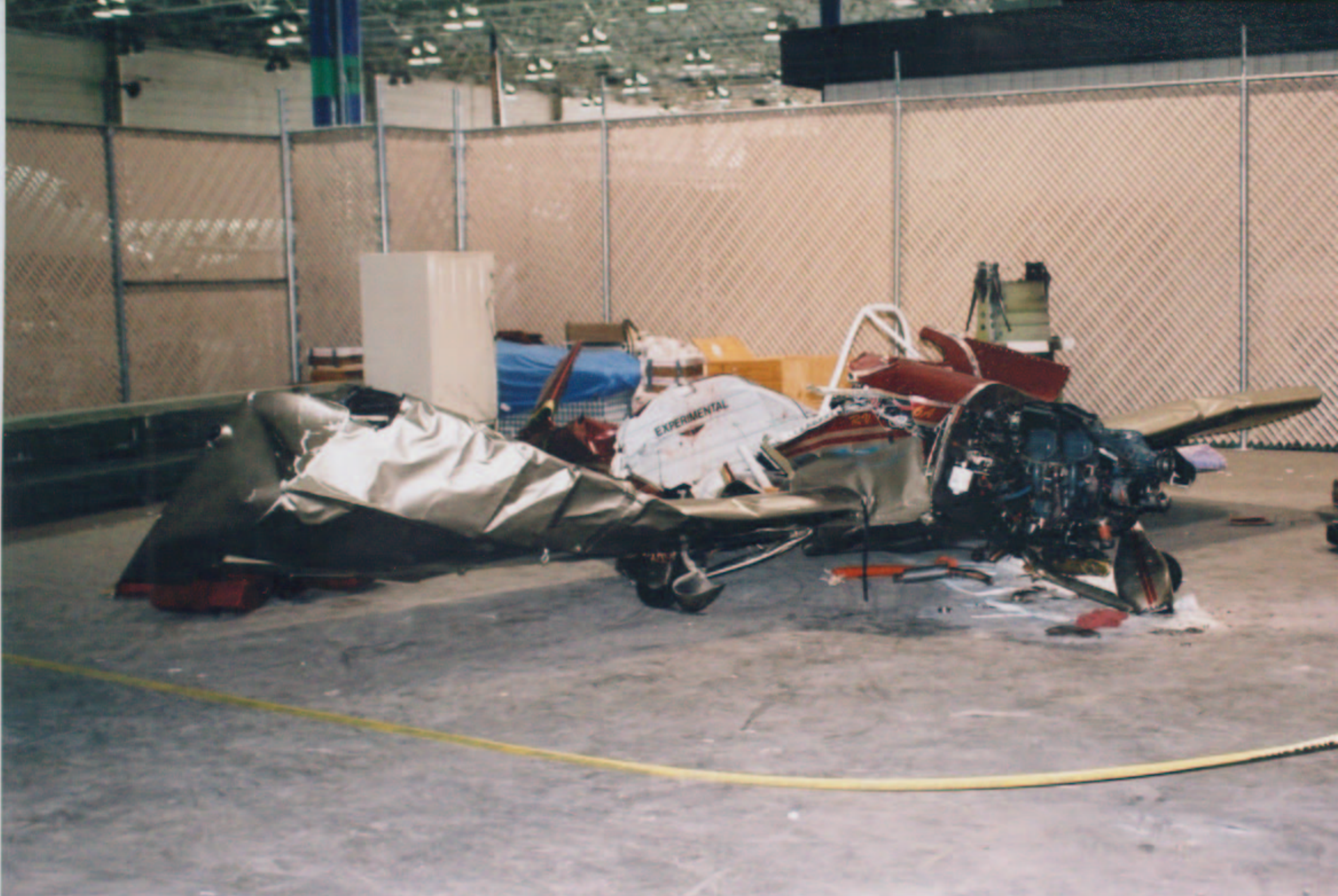
Photo 15 - View of N3333S landing edge of right wing and forward cabin area
