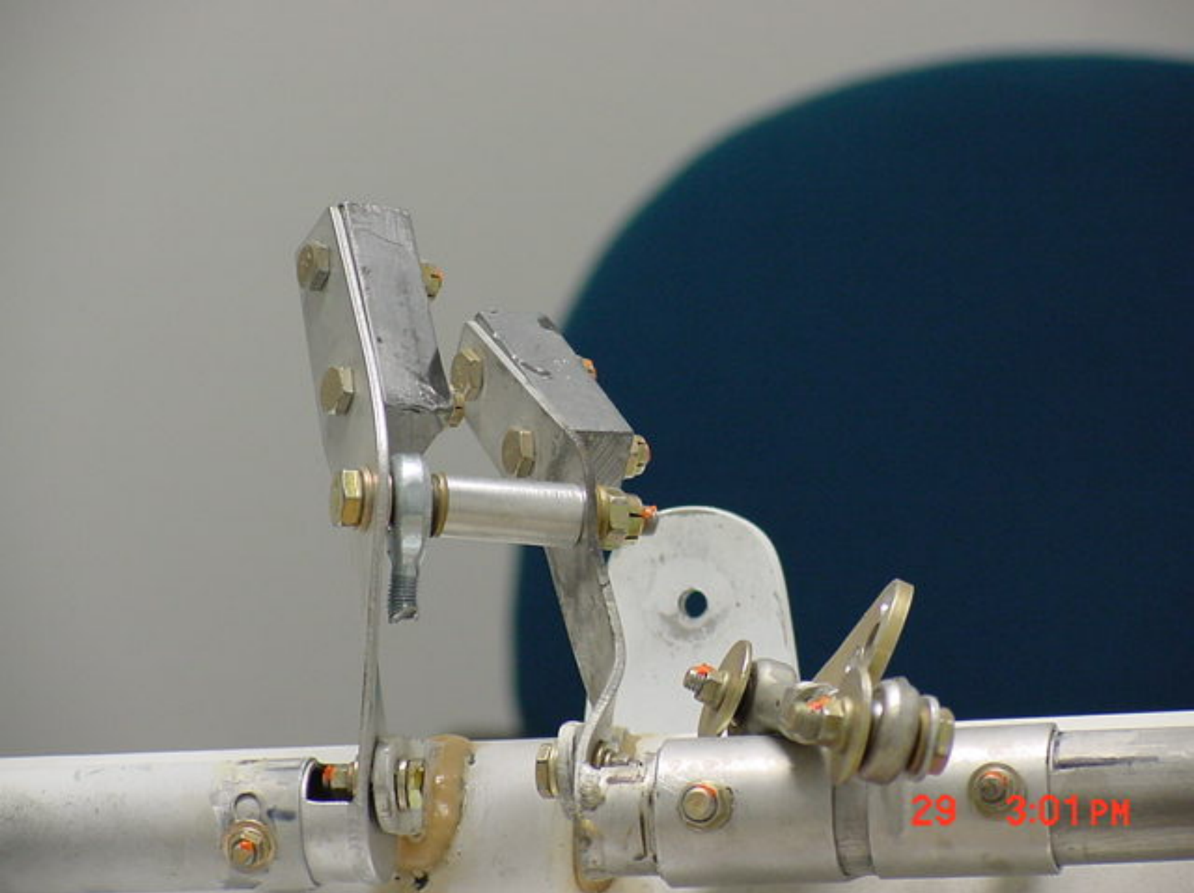
Photo 14. Canard Control Linkages
