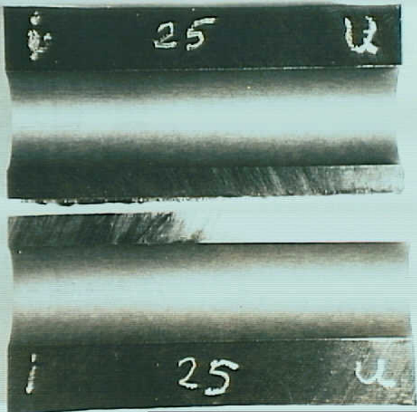
Photo 13. Hole #25 drilled with standard cutting data with HSS, fine bored and honed. BEA shows no indications.
