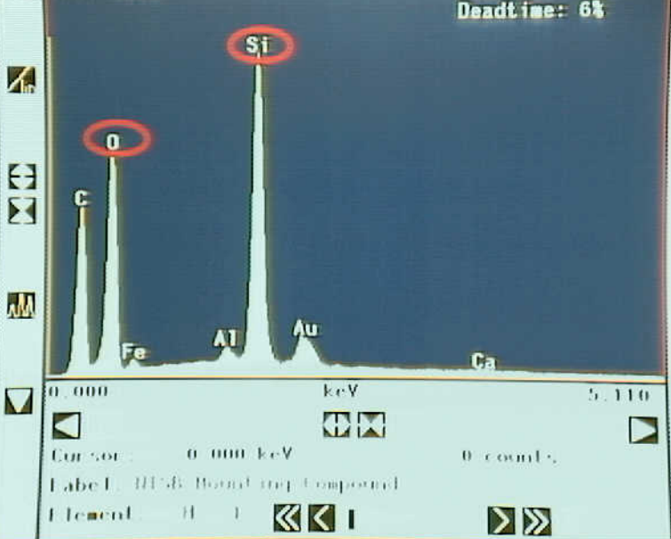
Photo 13. EDS spectrum taken from gold coated section of mounting compound. The oxygen and silicon peaks are identified.
