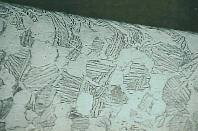
Photo 12. Cross section of hole #26 showing deformed material to a depth of up to 12 \mu\text{m} (0.47 mills). Mag 500X.
