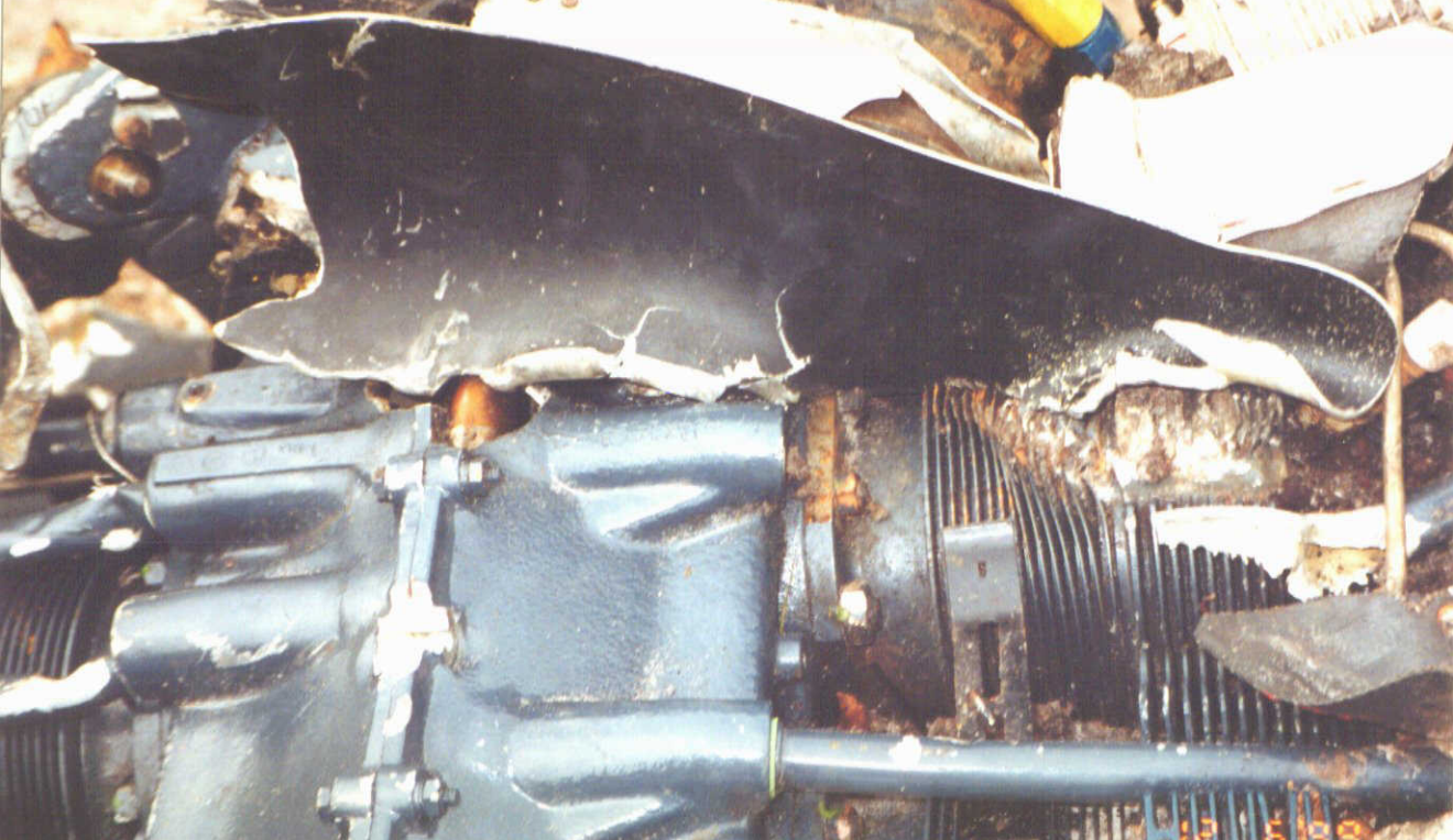
Photo 12: Closer view matching the impact signatures of the leading edge of the fractured propeller blade from the left propeller of the Seminole to the top of the engine from the Cadet
