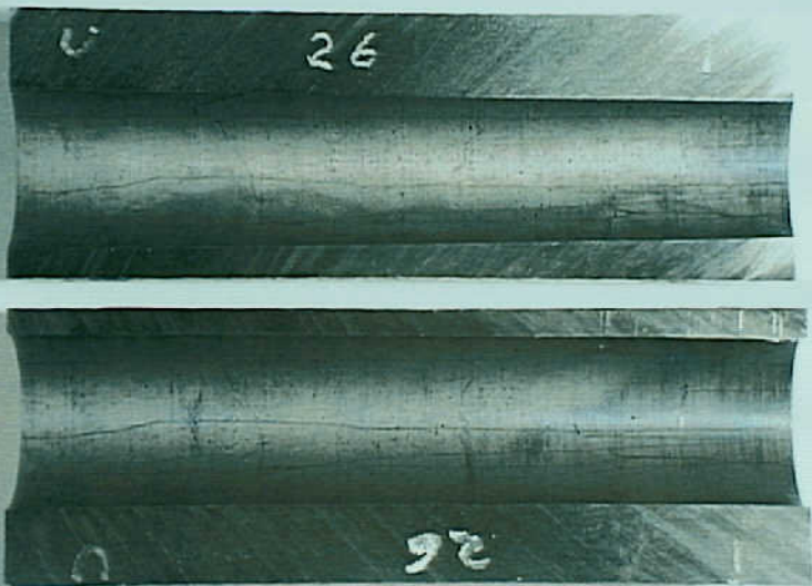
Photo 11. Hole #26 drilled with standard cutting data with HSS and fine bored. No indications came up to view a tBEA.
