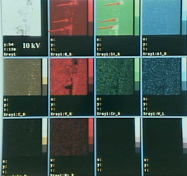
Photo 11. EDS map of Region 7, Figure 8. K-bank oxygen and silicon (arrows) were observed on the regions of low intensity backscatter electron return.
