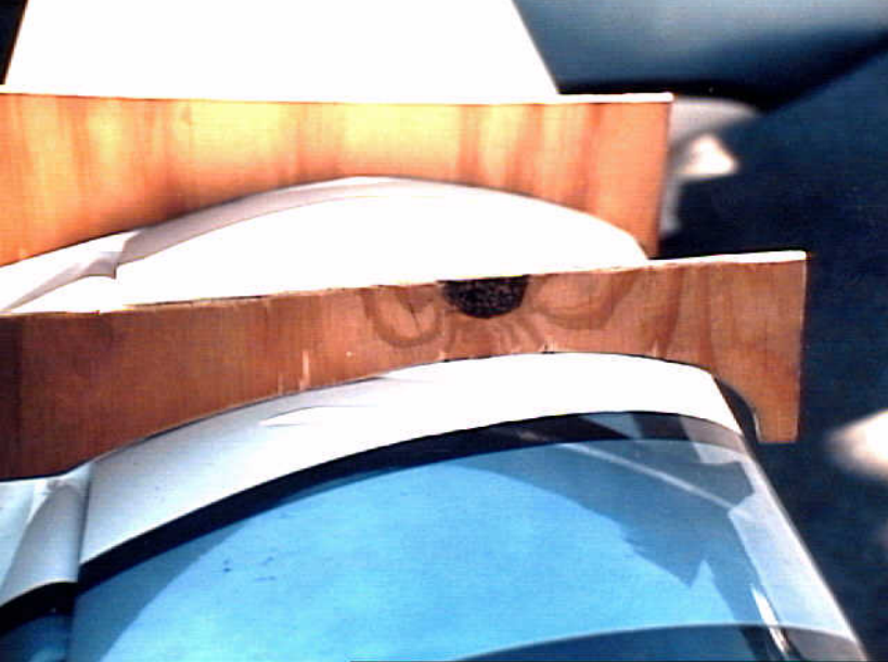
Photo 11. Airfoil templates forward is GU-25, aft is Ronz No. 1145MS.
