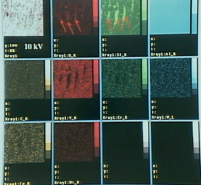
Photo 10. EDS map of the directional marring found in Region 6, Figure 8. K-bank oxygen and silicon were identified in the marred regions.
