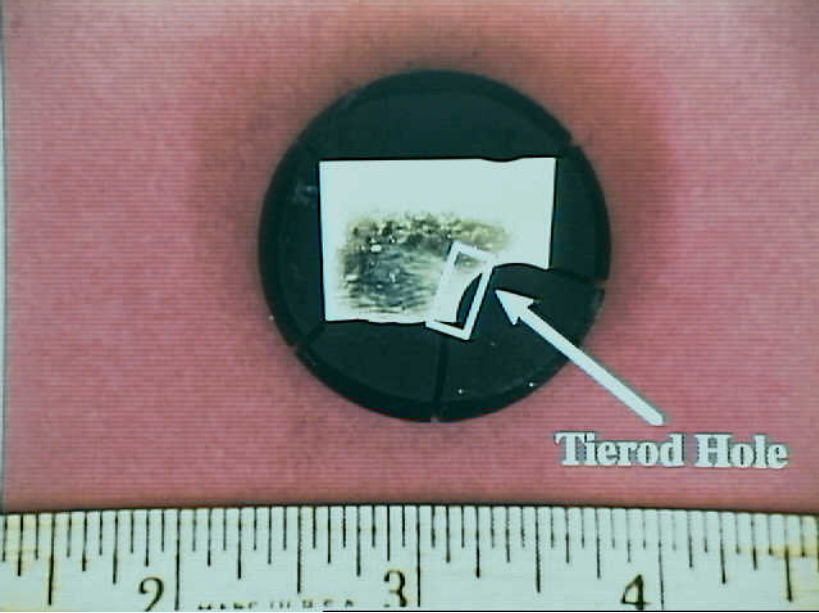
Photo 1. Mounted Specimen. Mounting material was cut before removal for SIMS analysis. The tierod hole is identified. The boxed region contains the fracture origin and the "hardened layer".
