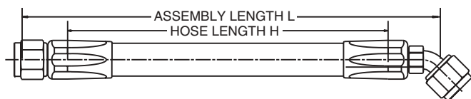
Straight-To-45° Elbow
