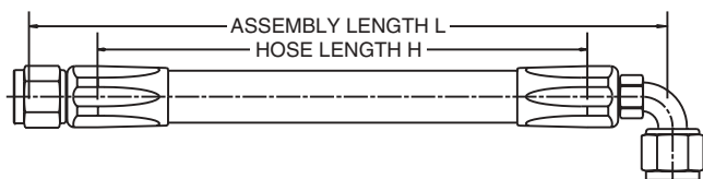
Straight-To-90° Elbow
