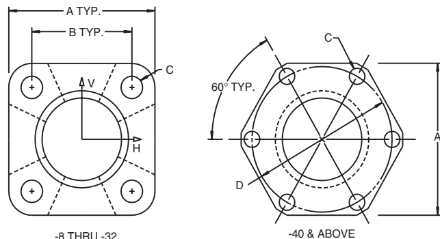
MS20756 Flange
