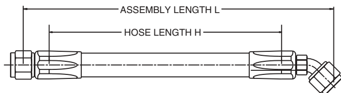
Straight-To-45° Elbow
