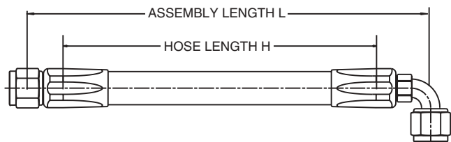
Straight-To-90° Elbow
