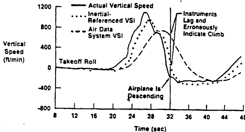
Figure 24. VSI error during takeoff windshear encounter. VSI may lag actual flight path changes.
