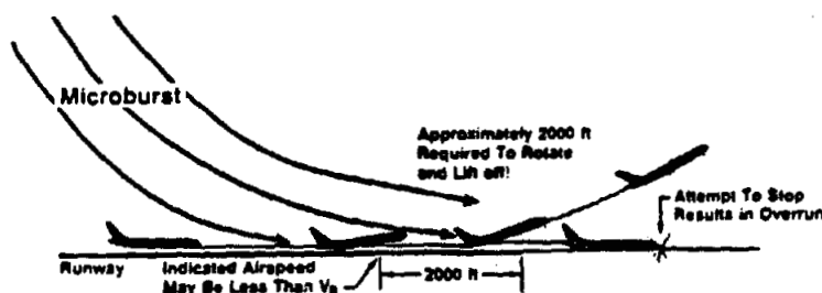
Figure 28. Windshear effects on rotation decision. Windshear effects may force rotation at speeds below V 1 . Rotation should begin no later than 2000 ft from runway departure end.
