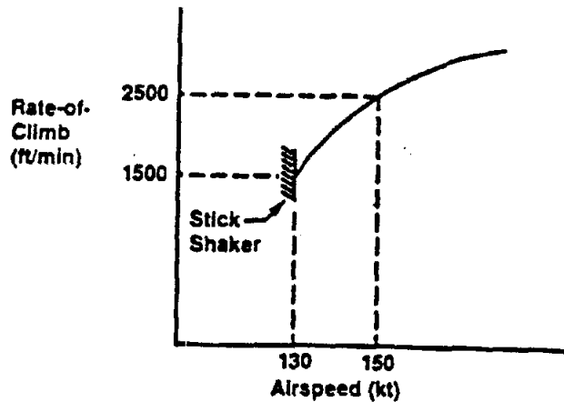
Figure 23. Typical takeoff rate-of-climb capability. Significant climb capability exists even at stick shaker airspeeds.
