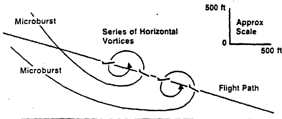
Figure 22. Encounter with microburst horizontal vortices. Rapid updraft downdraft variations due to horizontal vortices can cause uncommanded pitch changes and may result in momentary stick shaker activation well above normal stick shaker speeds.
