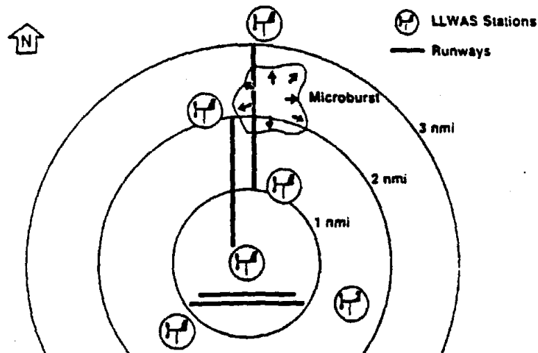
Figure 26. Undetected microburst due to wide LLWAS station spacing
