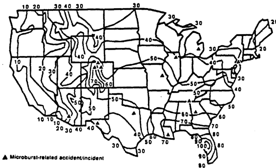
Figure 6. Average annual continental U.S. thunderstorm days. Correlation exists between regions of higher thunderstorm activity and windshear-related accidents/incidents
