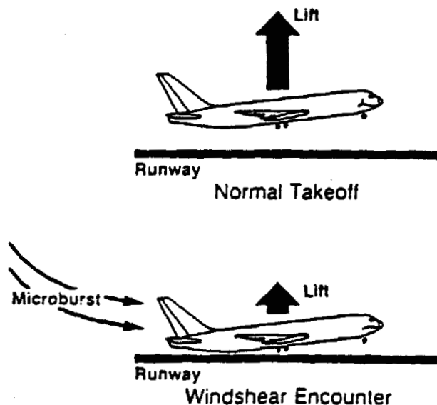
Figure 18. Windshear effects on liftoff. Microburst reduces airspeed and lift at normal attitude that results in inability to lift off.
