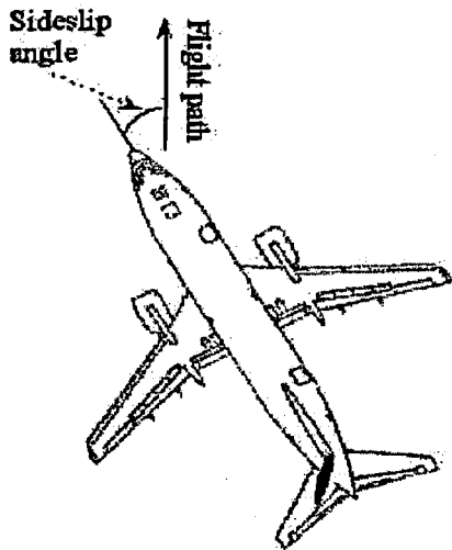
Figure 1 Rudder Induced Sideslip
