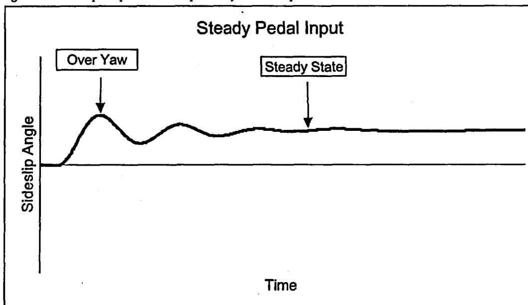
Figure 2 "Sideslip Response to Abrupt Steady Rudder Input"
