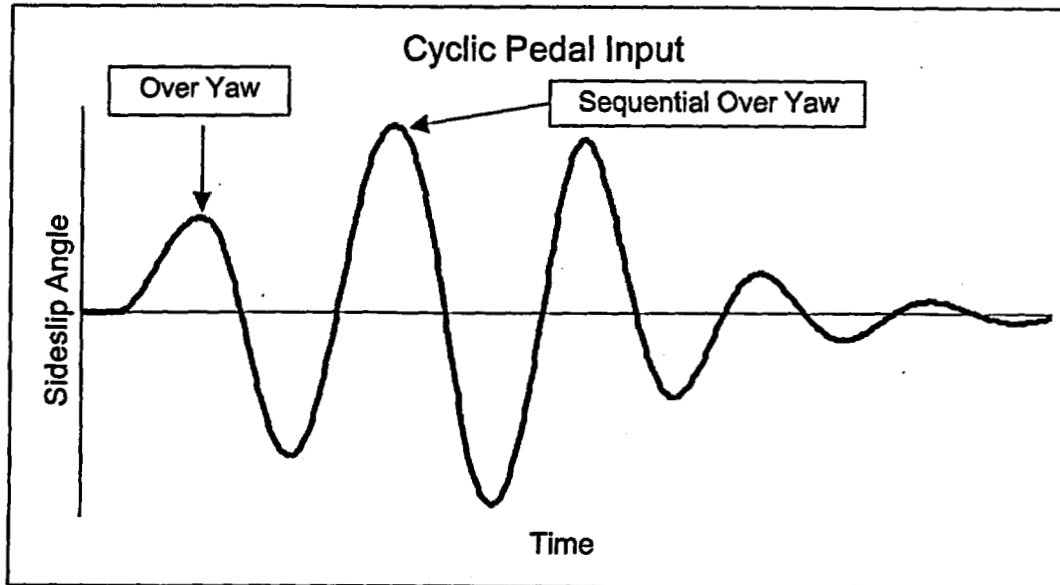
Figure 3 "Sideslip Response to Abrupt Cyclic Rudder Input"
