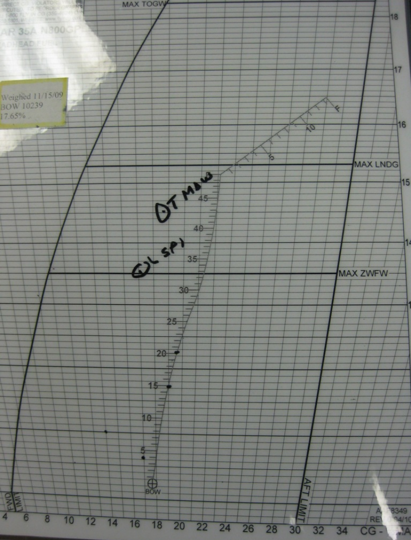
Board Weight & Balance -- Accident Flight
