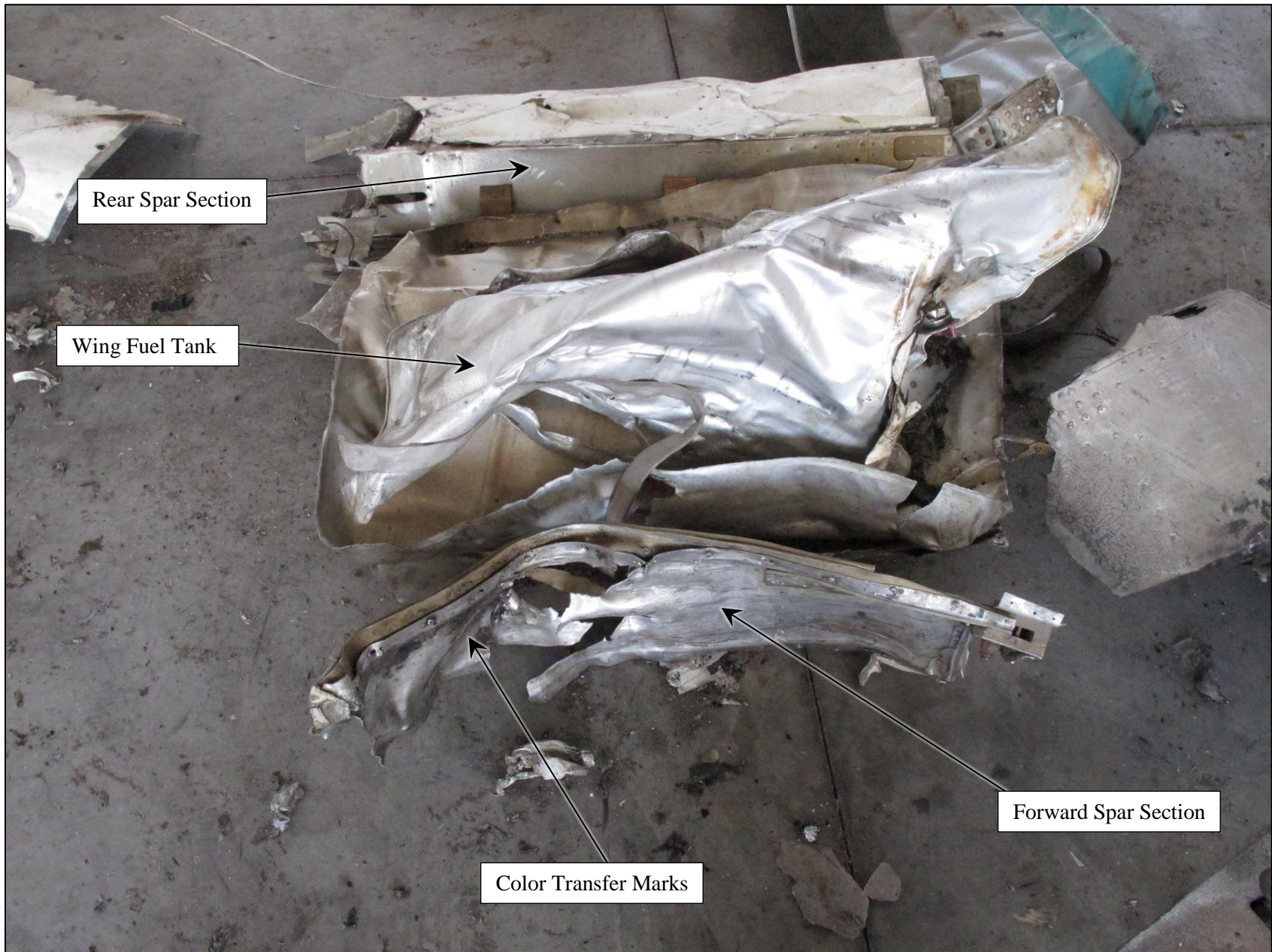
Photo 10 - Cessna Right Wing Forward Spar Section
