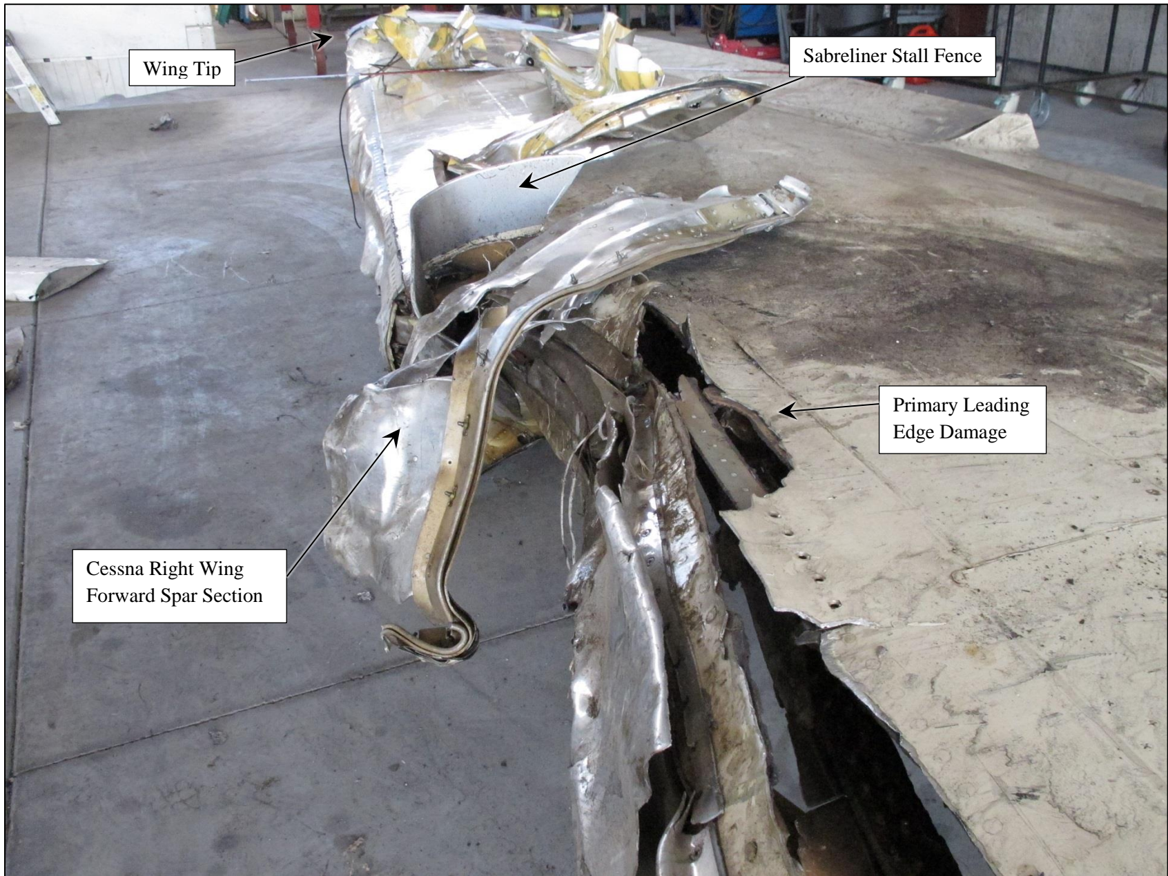
Photo 11 – Sabreliner Right Wing and Cessna Right Wing Forward Spar Section
