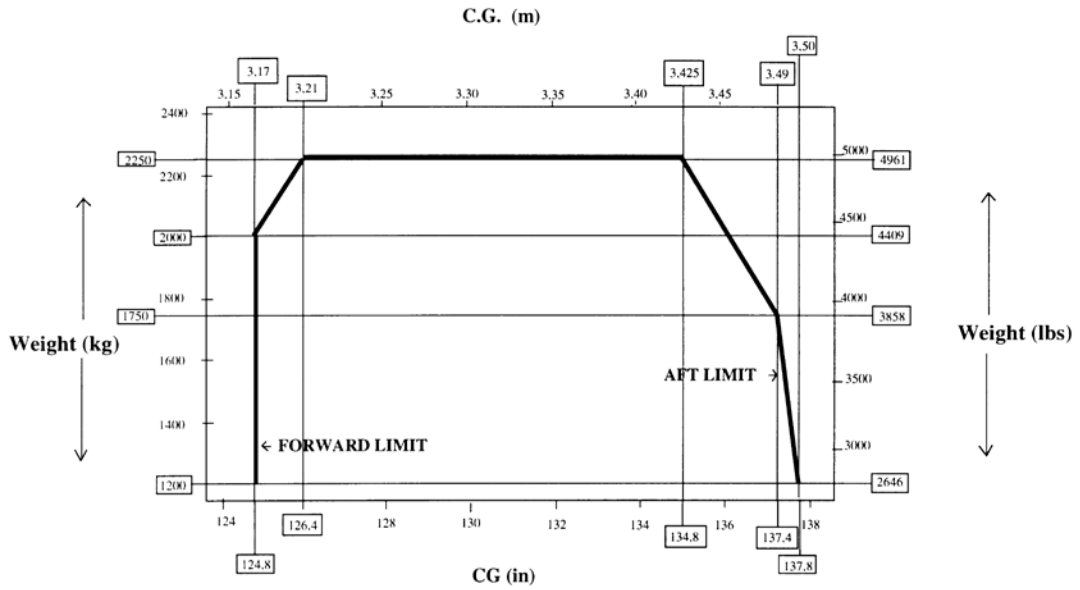
Longitudinal: AS350 B3 ARRIEL 2B (after modifications AMS 072803 and 072808):
