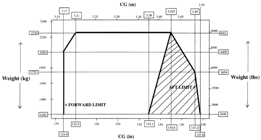
Longitudinal: AS350 B3 ARRIEL 2D a/c incorporating mod. OP-3369:
