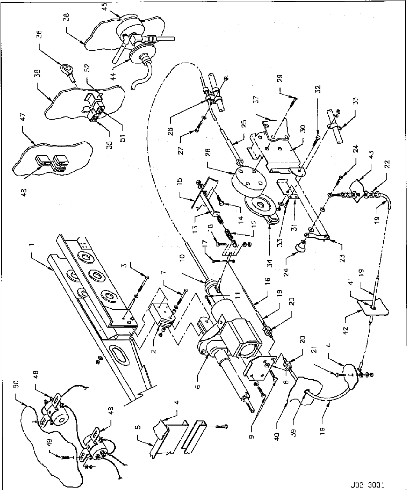
FIGURE 2 - EMERGENCY EXTENSION SYSTEM & ACTUATOR INSTL. S/N 24-0001 THRU 24-0083, 24-0085 THRU 24-0377
