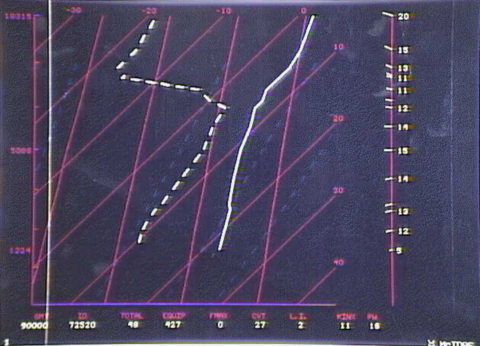
Meteorology 5A - Attachment six - Skew-T Log-P Diagram
