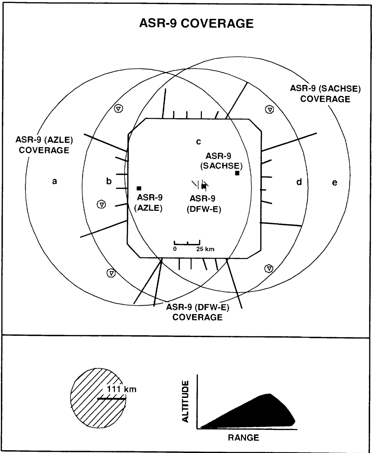
Figure 4. Location and coverage regions for the three ASR-9 radars used in the DFW ITWS precipitation-with-AP-removed product. In areas where data from two radars overlap, the higher value is used, and in areas where data from three radars overlap, the median value is used. Regions (a) and (e) have single ASR-9 coverage. Regions (b) and (d) have dual coverage, and region (c) has triple coverage. The lower Figure shows a plan view of the scanning range and a vertical cross section of the fan beam coverage of each of the ASR-9 radars.
