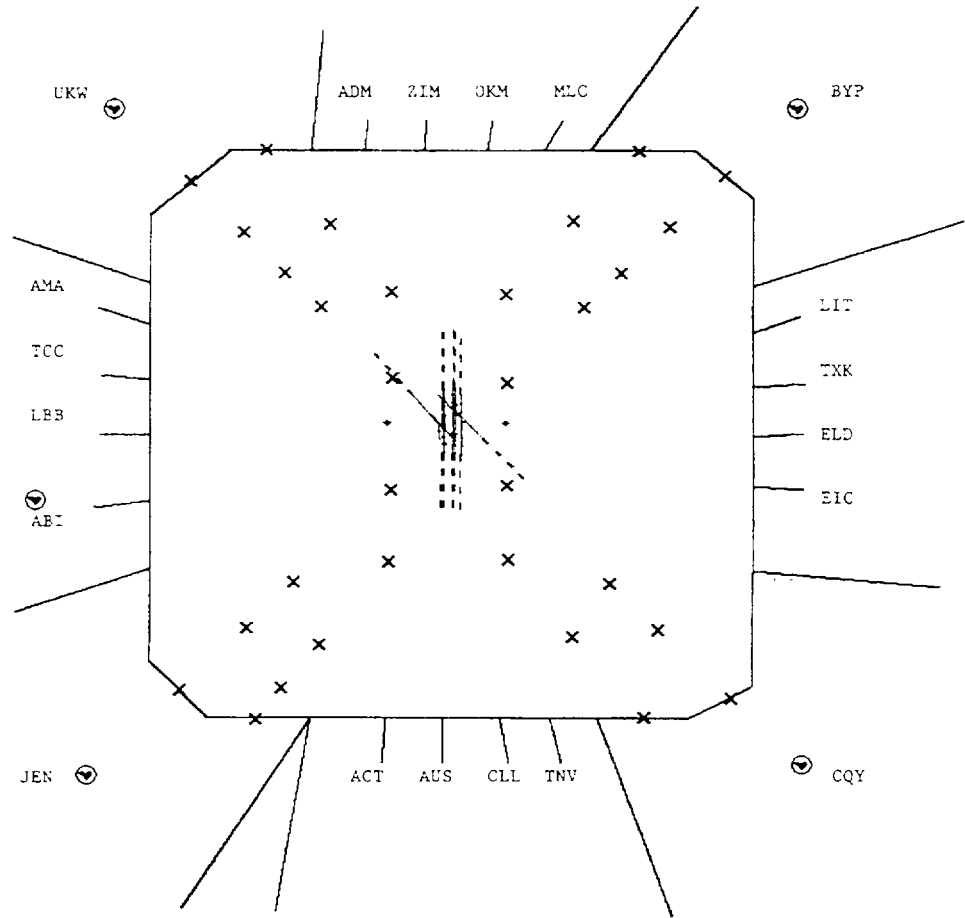
Figure A-1. DFW TRACON with standard jet arrival and departure fixes.
