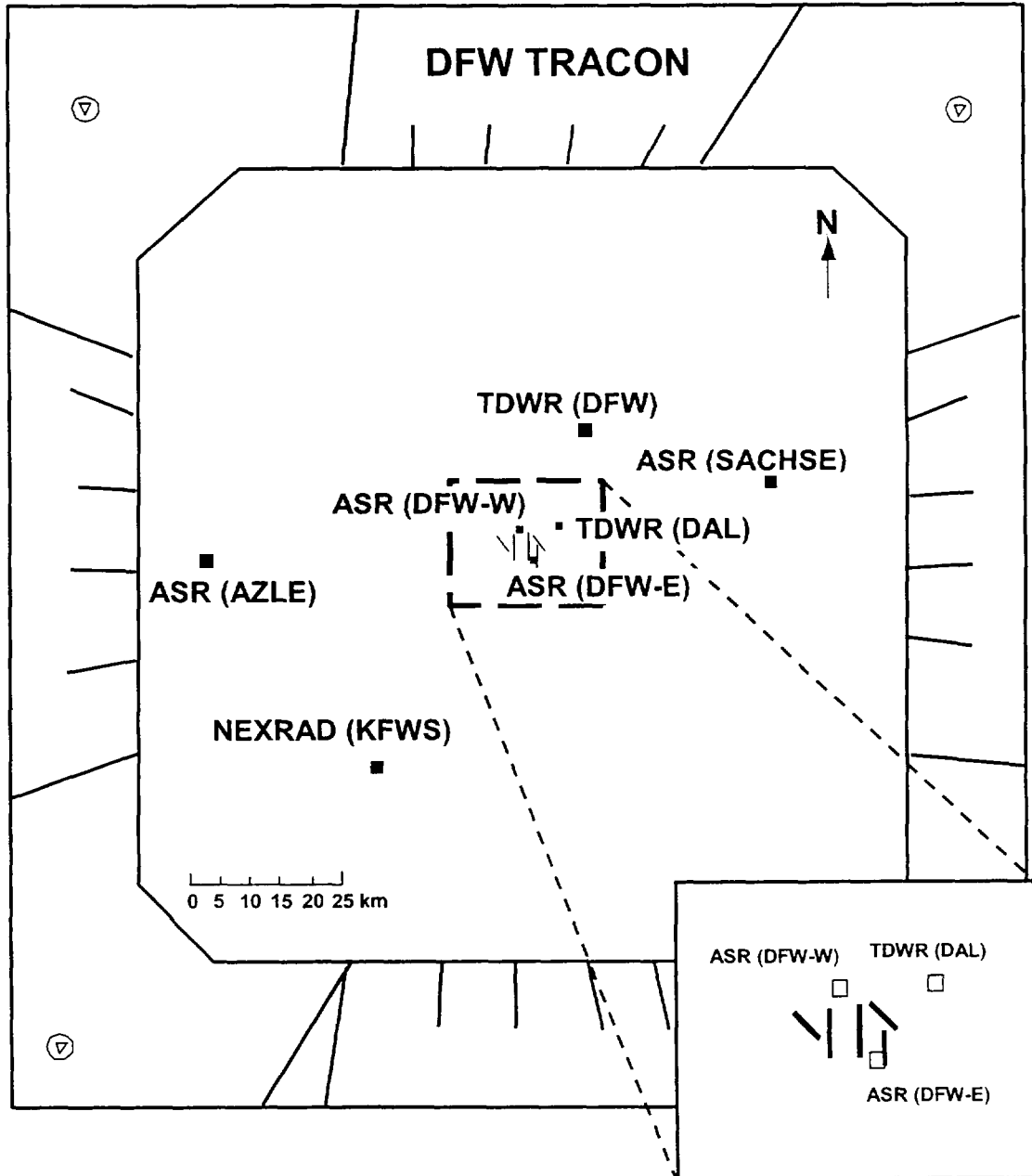
Figure 1. DFW Terminal Radar Approach Control (TRACON) airspace and weather sensor locations.
