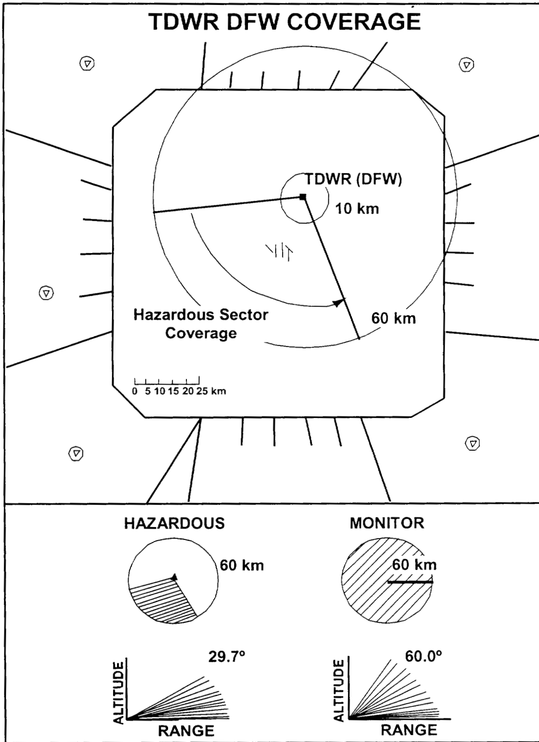
Figure 8. The location and coverage region for the DFW TDWR. Data were used beyond 10km and within 60 km of the radar. The lower Figure shows a plan view of the scanning range and a vertical cross section of the scan strategy for the radar in "hazardous" and "monitor" modes.
