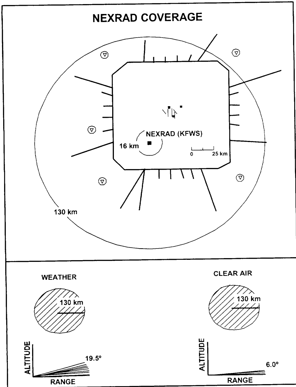
Figure 6. KFWS NEXRAD location and coverage region. In this study, reflectivity data were used for the regions between 16 km and 130 km from the radar. Data closer than 16 km were not used because the data in that region do not extend to an altitude of at least 6 km. The lower Figure shows a plan view of the scanning range and a vertical cross section of the scan strategy for both "weather" and "clear-air" modes.
