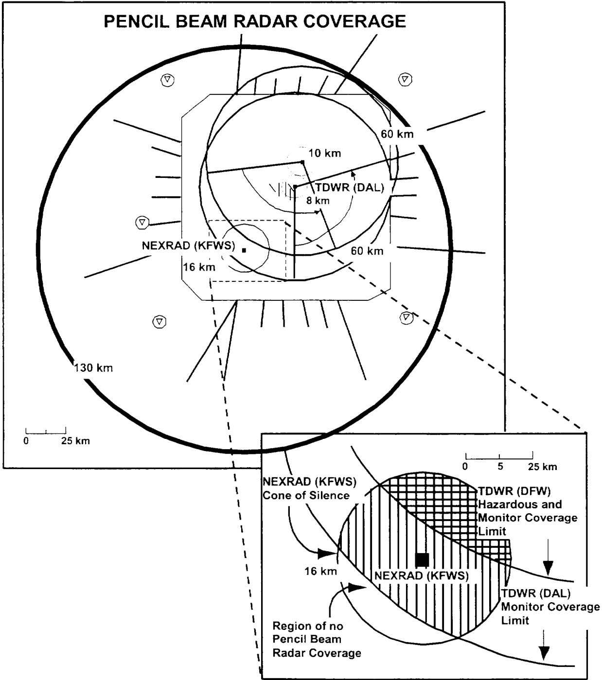
Figure 14. Pencil-beam radar coverage regions inside the TRACON.
