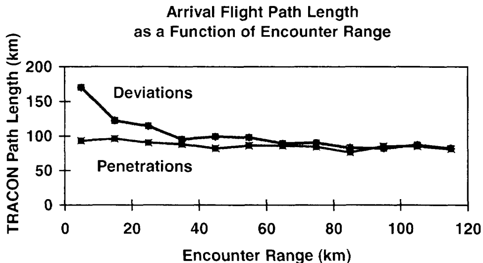
Figure 20. Pathlength flown inside the TRACON as a function of encounter range. Aircraft that deviate within 25 km of the airport fly longer pathlengths on average than aircraft that penetrate. There is very little pathlength penalty, on average, for deviating around storms farther away from the airport.
