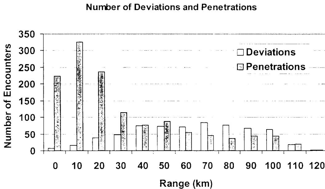
Figure 15. Histogram of the number of penetrations and deviations as a function of range.
