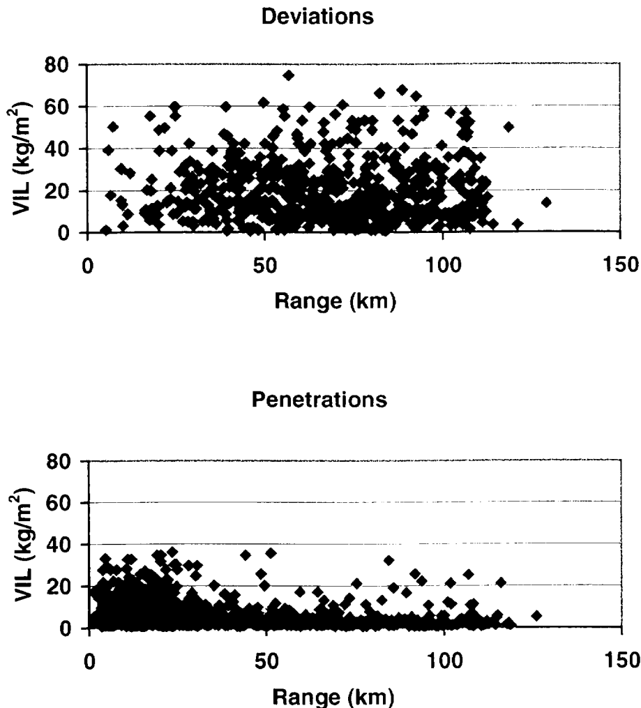
Figure 19. Penetrations and deviations as a function of range and VIL. There are very few penetrations of high VIL values far away from the airport. There are very few deviations near the airport regardless of VIL value.
