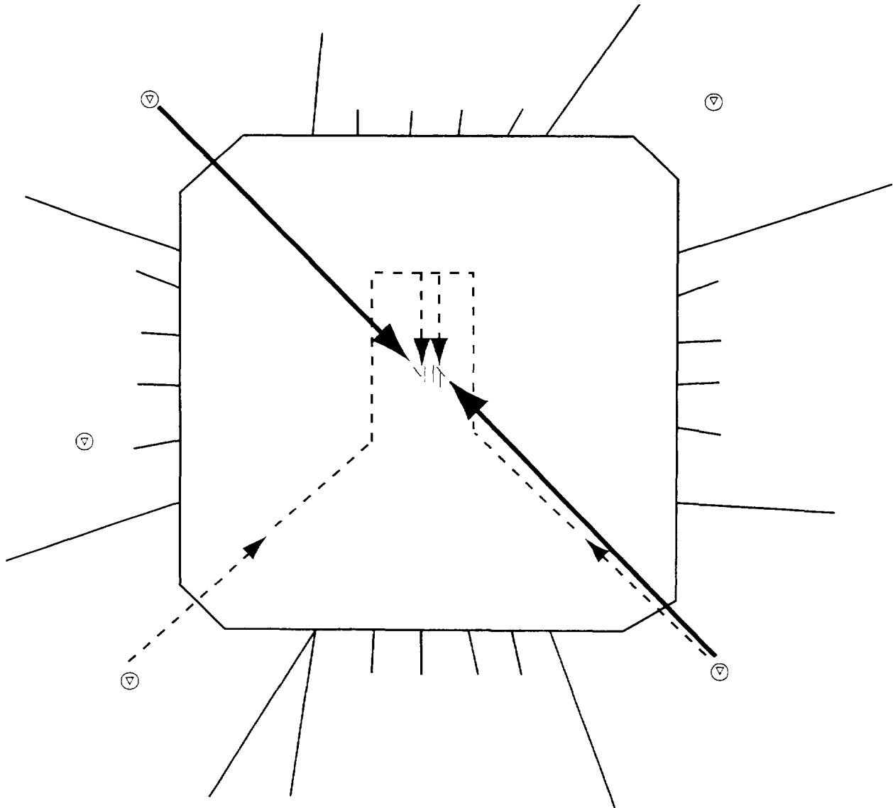
Figure 22. Flightpaths of aircraft included in the hypothesis test. The solid black lines represent aircraft that flew straight from the northwest and southeast cornerposts to their destination runways. The dashed lines represent aircraft arriving from the south that needed to turn in order to execute downwind and final legs of flight before landing.
