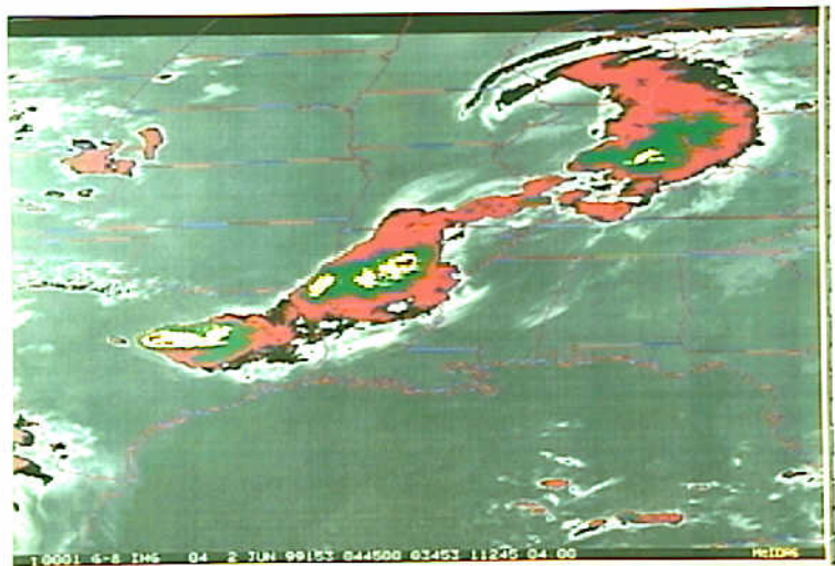
Meteorology 5 - Exhibit No. 5B - Attachment 42 - Infrared satellite image at 0445Z.
