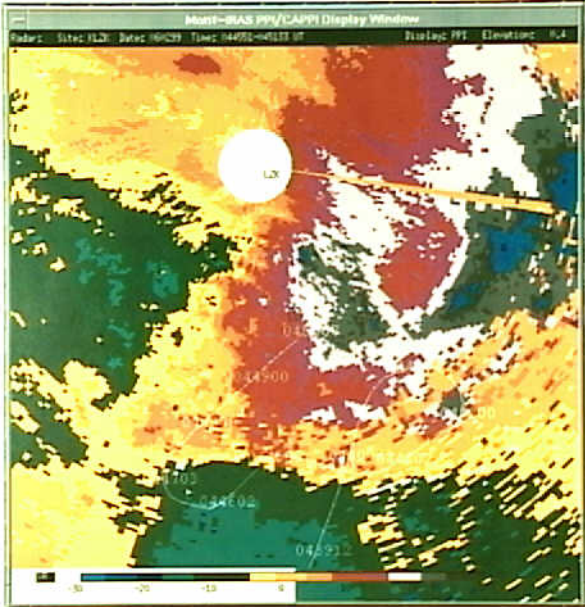
Meteorology 5 - Exhibit No. 5B - Attachment 26 - WSR-88D radial velocity for 0.4 degrees at 0451Z.
