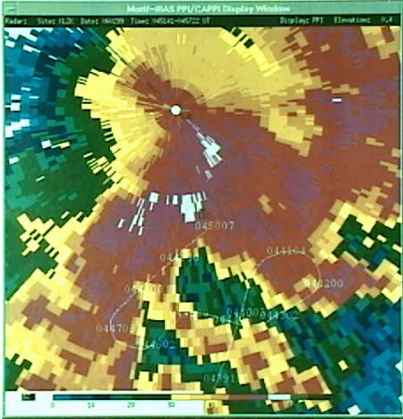
Meteorology 5 - Exhibit No. 5B - Attachment 19 - WSR-88D base reflectivity for 1.5 degrees at 0451Z.
