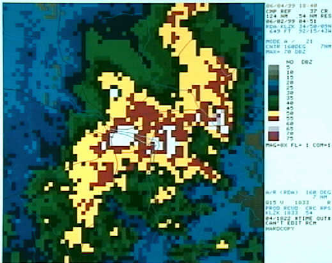
Meteorology 5 - Exhibit No. 5B - Attachment 15 - Composite reflectivity at 0451Z.
