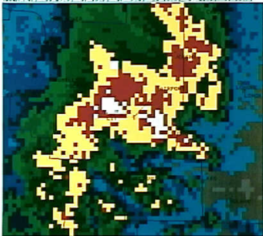
Meteorology 5 - Exhibit No. 5B - Attachment 14 - Composite reflectivity at 0445Z.
