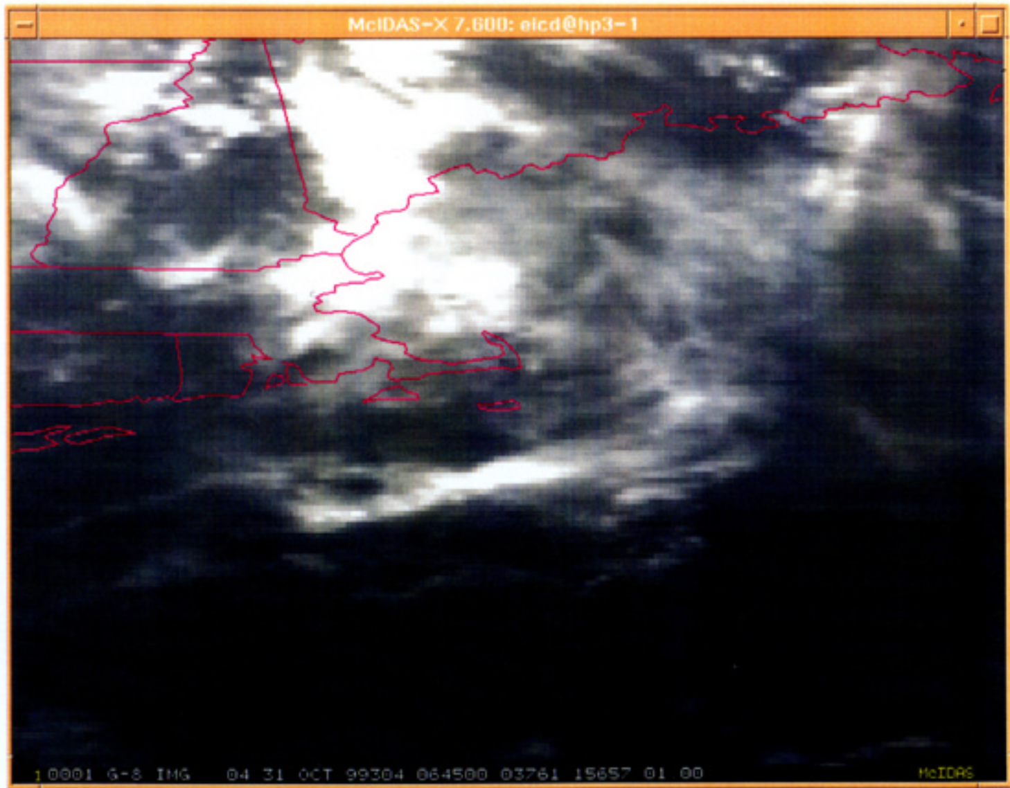
Attachment 8 Infrared Satellite image at 0645Z
