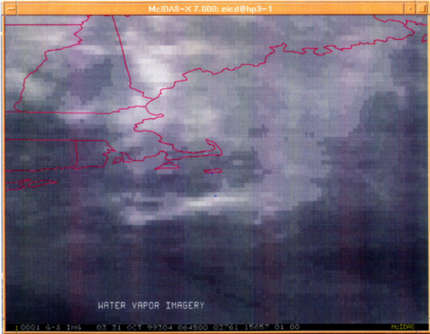
Attachment 10 Water vapor satellite image at 0645Z
