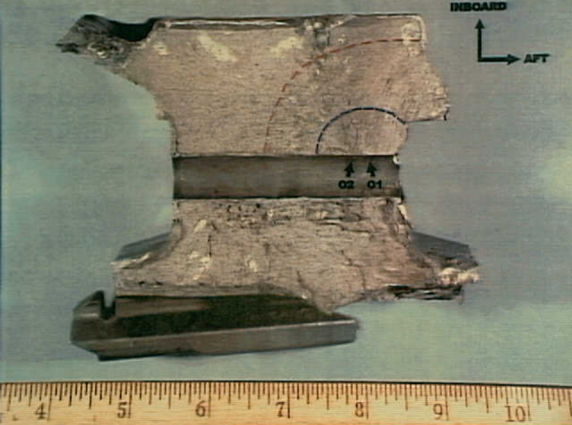
Materials Laboratory 15 - Photo 1. Photograph of Exhibit No. 15D
