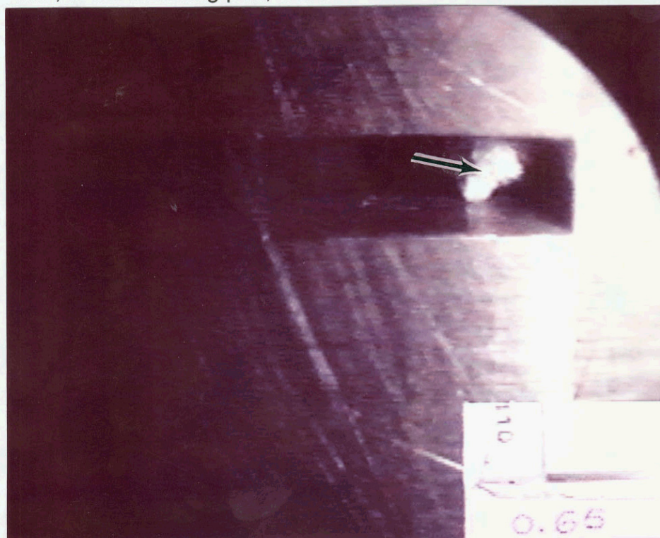
Figure 36. Particle (arrowed) found in the Pa to C4 metering port on the inside diameter of S/N 2956 secondary slide. Approximately X50.
