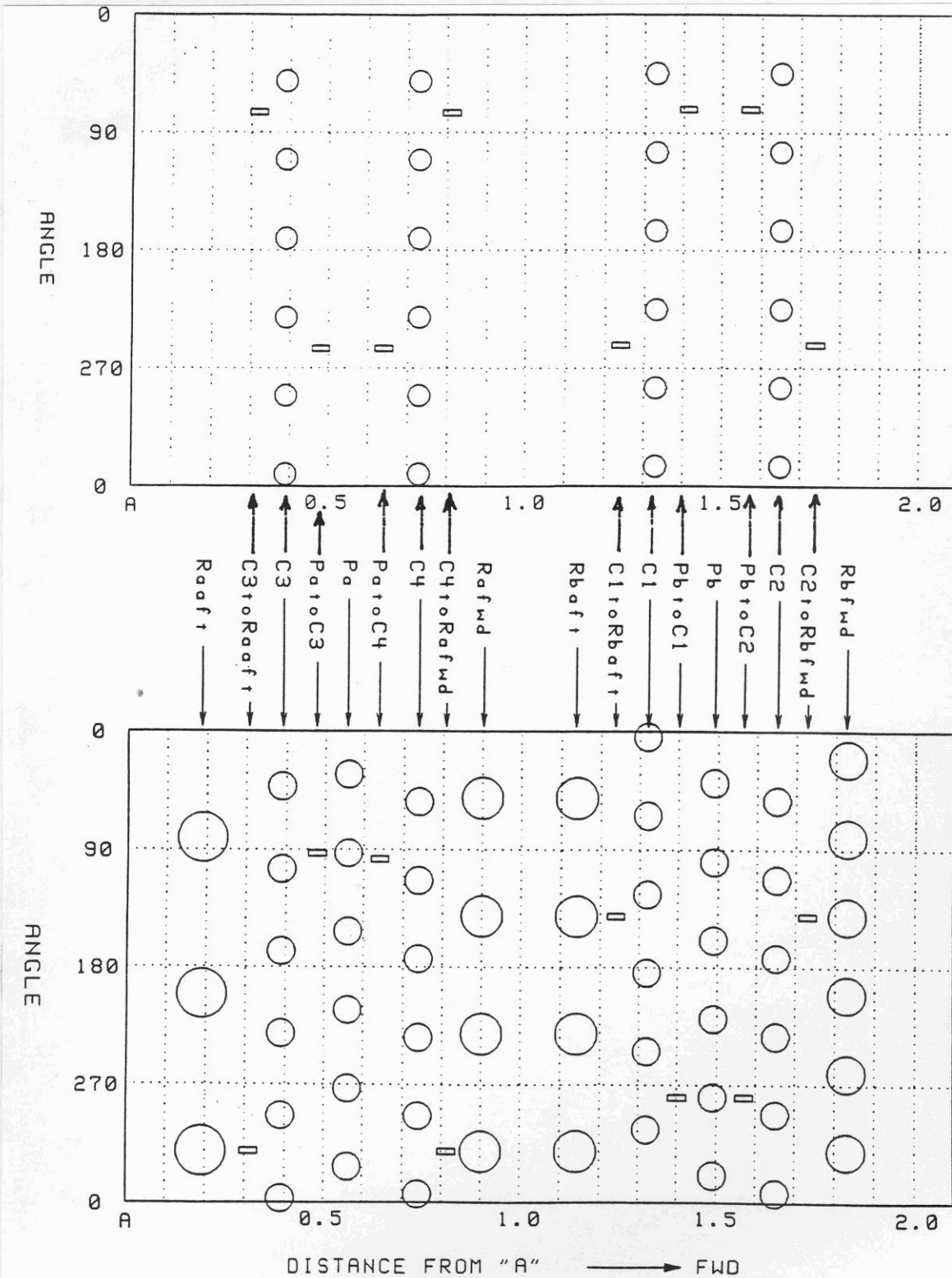
Above views indicate the relative sizes and positioning of the round holes and rectangular metering ports of the secondary (top view) and housing (lower view). Holes, ports and distances only are approximately to scale (about X2.5). The vertical distances for the angular positions are not to the same scale (illustration only).
