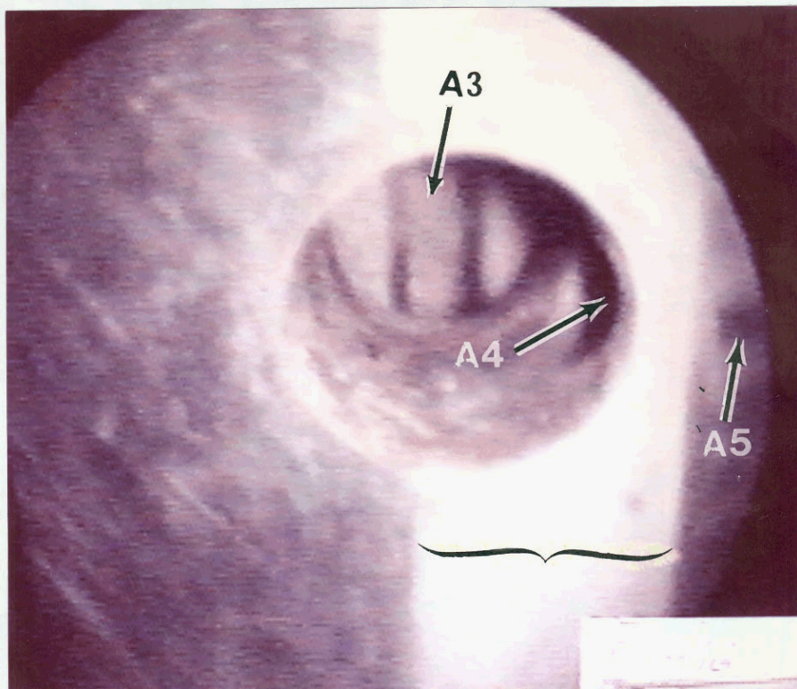
Figure 35. The Ra aft hole in the S/N 1091 housing illustrating the light banding (bracket), the annulus, "A3", and the side hole, "A4", to the metering port, "A5".
