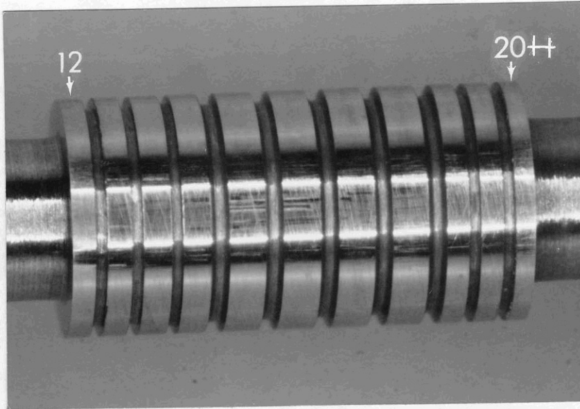
Figure 3. Another area showing a high concentration of burnishing marks. Exemplar 2108X primary, lands 12 to 20++ at 30 degrees. X7.5
