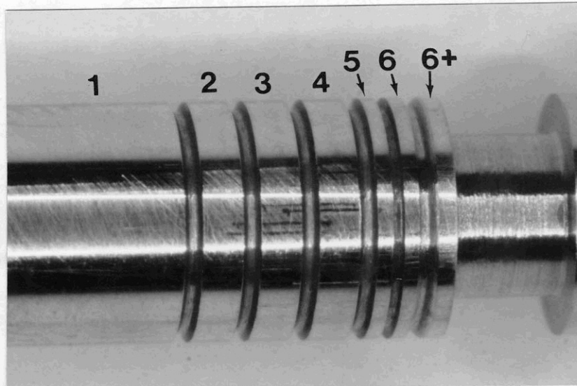
Figure 1. Primary for exemplar 2108X showing a location of concentrated burnishing marks. Lands 1 through 6+, reference angular position about 130 degrees. X7.5
