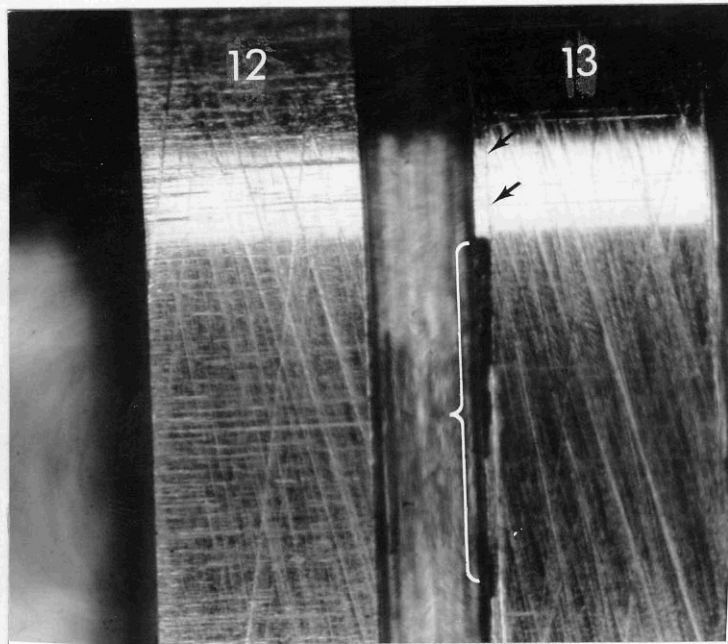
Figure 10. Larger chip out area (bracket area) of the land / balance groove corner found on exemplar 2108X at about 45 degrees for land 13 . Note circumferential mark located by arrowheads. X50
