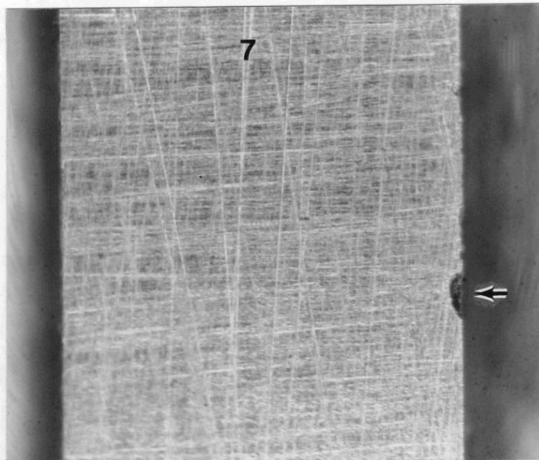
Figure 28. Small chip out of metering edge. Exemplar 2108X, land 7 at 10 degrees. X50
