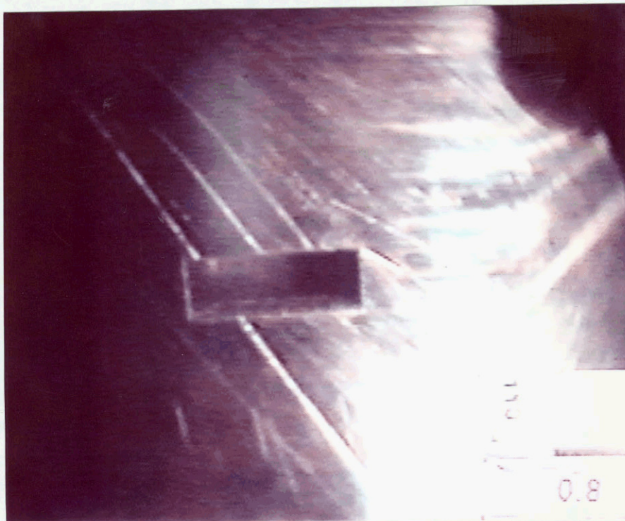
Figure 38. Scratches at the Pa to C4 metering port on the inside diameter of S/N 2567 secondary that would correspond to the approximate area containing the chip out and scratch on the primary shown in figure 37. X27
