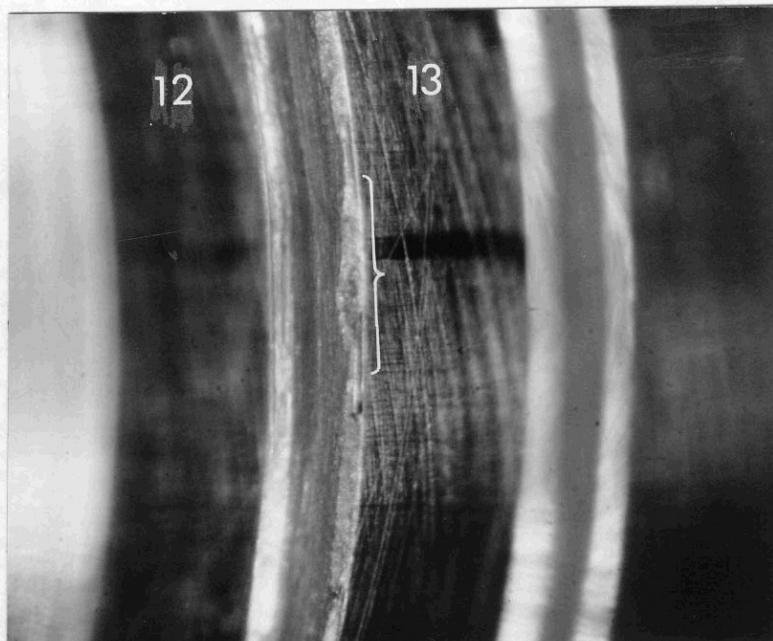
Figure 13. Same as that shown above except at higher magnification. Side wall of the balance groove is about 0.010 deep and the chipping was estimated to be about 0.003 inch along wall. X50
