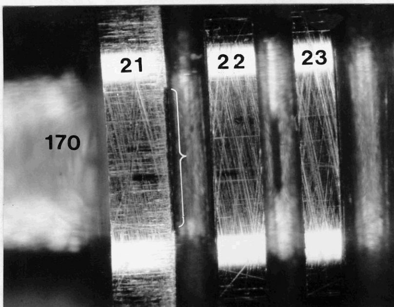
Figure 14. Three areas displaying corner chip outs (at brackets) along balance groove interface with land 21 on S/N 2108X exemplar. Reference angular position indicated to left of metering edge. All photos X50.
