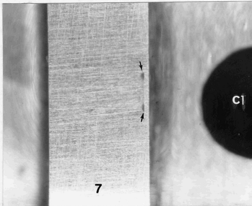
Figure 27. Probable witness mark (between arrows) on secondary outside diameter signifying the forward edge of the C1 to Rb aft metering port. Exemplar 2108X, land 7 at 110 degrees. X30
