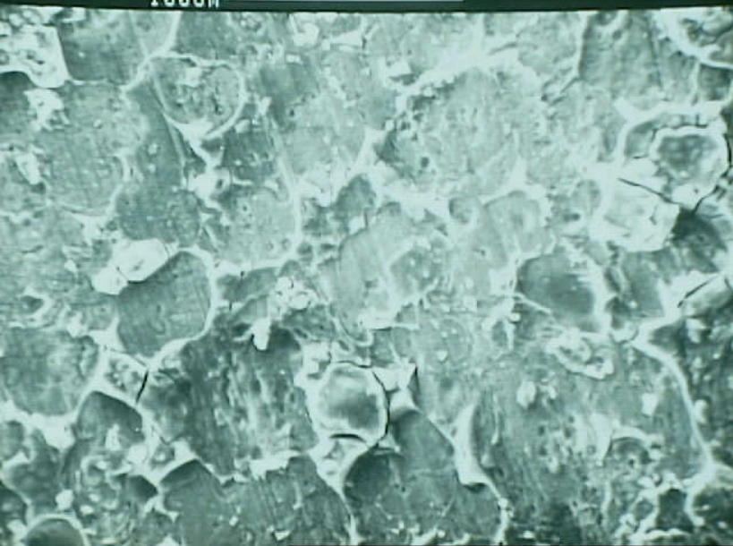
Materials Laboratory 15 - Exhibit No. 15B - Photo 5. SEM photograph of the features within the deformed crescent adjacent to the hole on the upper surface. Remnants of the mud-cracked oxide deposits are also visible on the surface. (334X)
