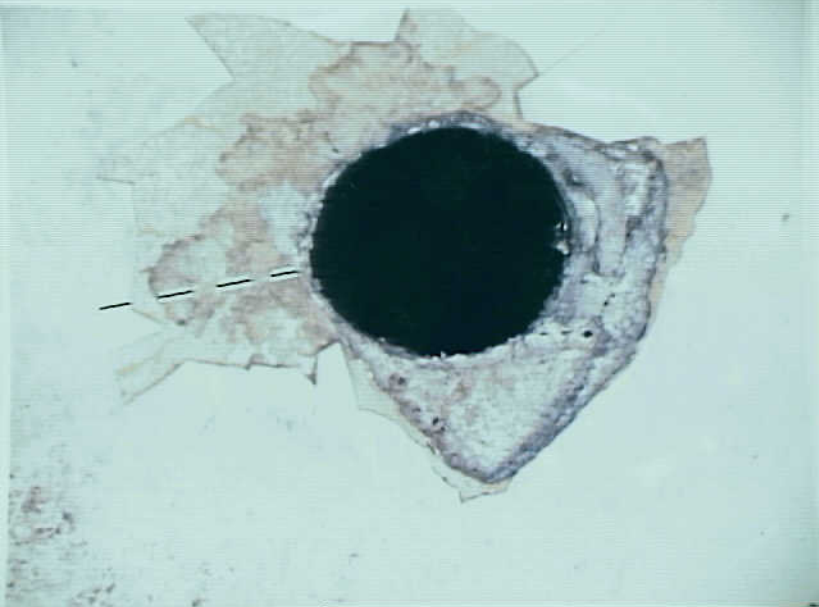
Materials Laboratory 15 - Exhibit No. 15B - Photo 4. Closer view of the hole, as shown from the lower surface of the piece. (7.5X)
