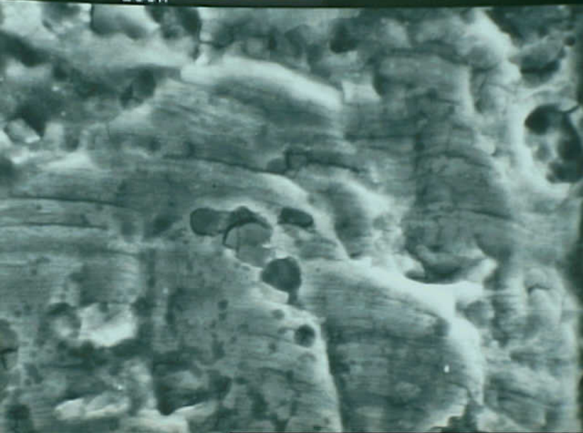
Materials Laboratory 15 - Exhibit No. 15A - Photo 6. SEM photograph of a fracture area containing a fatigue striation pattern. (1,330X)
