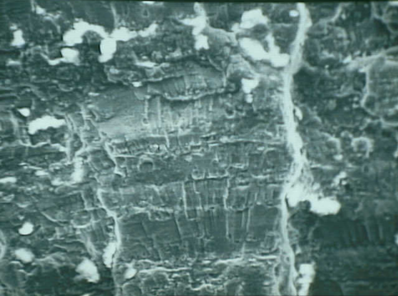
Materials Laboratory 15 - Exhibit No. 15A - Photo 3. SEM photograph showing ratchet marks separating origin areas along the fillet radius (at the bottom of the photograph) and the fatigue banding pattern adjacent to the radius. (134X)
