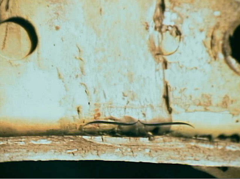
Materials Laboratory 15 - Exhibit No. 15A - Photo 1. View looking forward at a portion of the front spar lower chord fracture. The bracket indicated the location of a fatigue crack.
