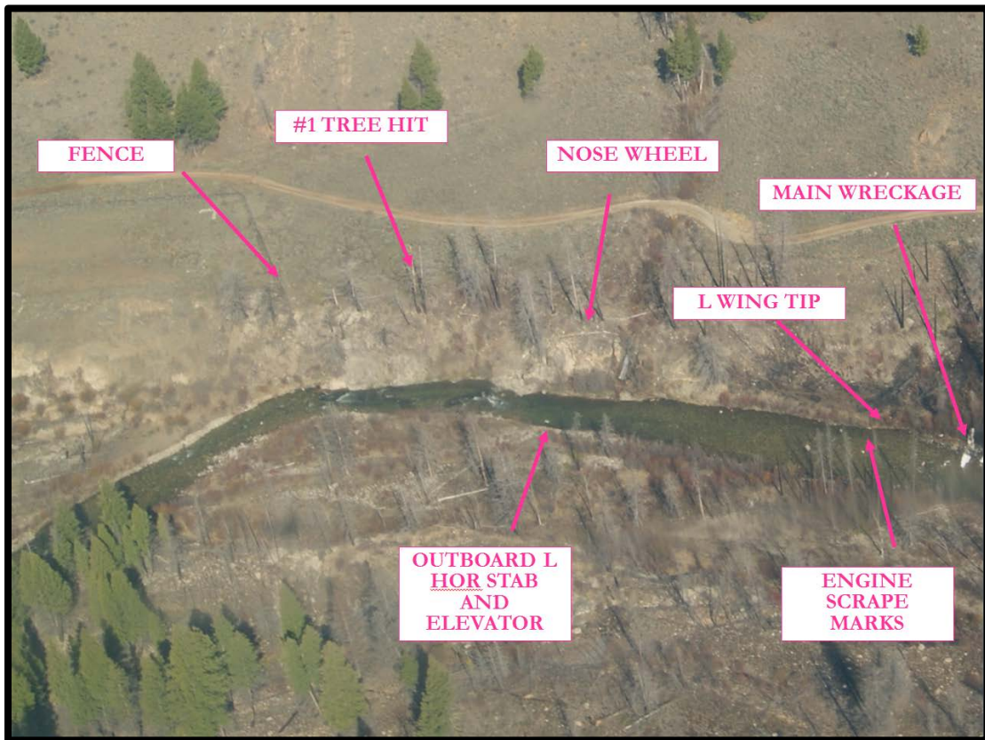
Picture 8: The Main Wreckage with Respect to the Terrain and River
