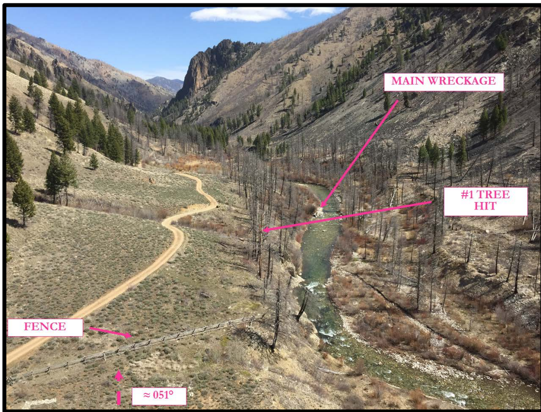
Picture 6: The Main Wreckage with Respect to the Tree
