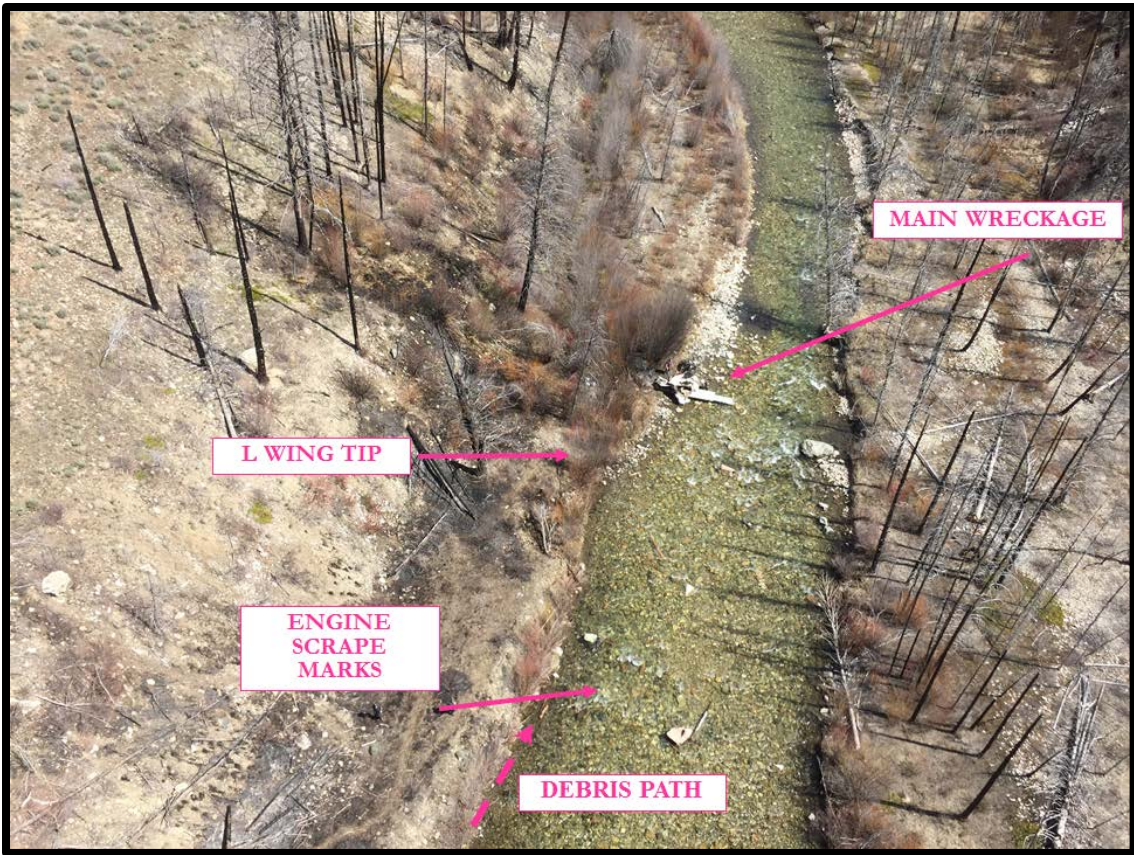
Picture 7: The Main Wreckage with Respect to the Debris Field
