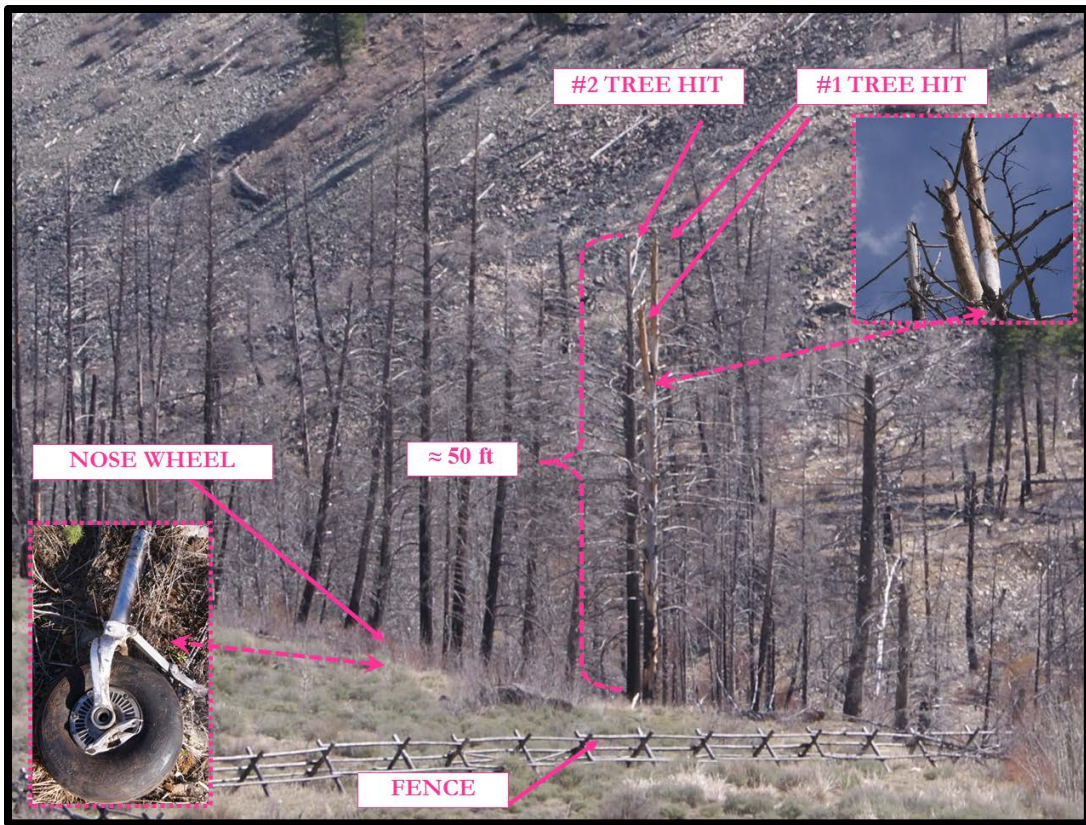
Picture 11: The Trees (first impact) and Nose Wheel
