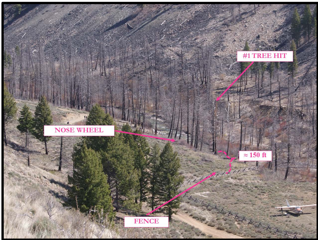
Picture 10: The Main Wreckage with Respect to the Fence
