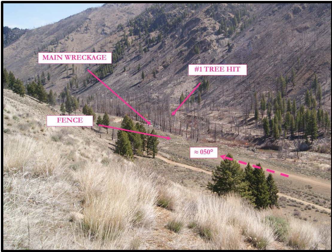
Picture 9: The Main Wreckage with Respect to the Tree Line
