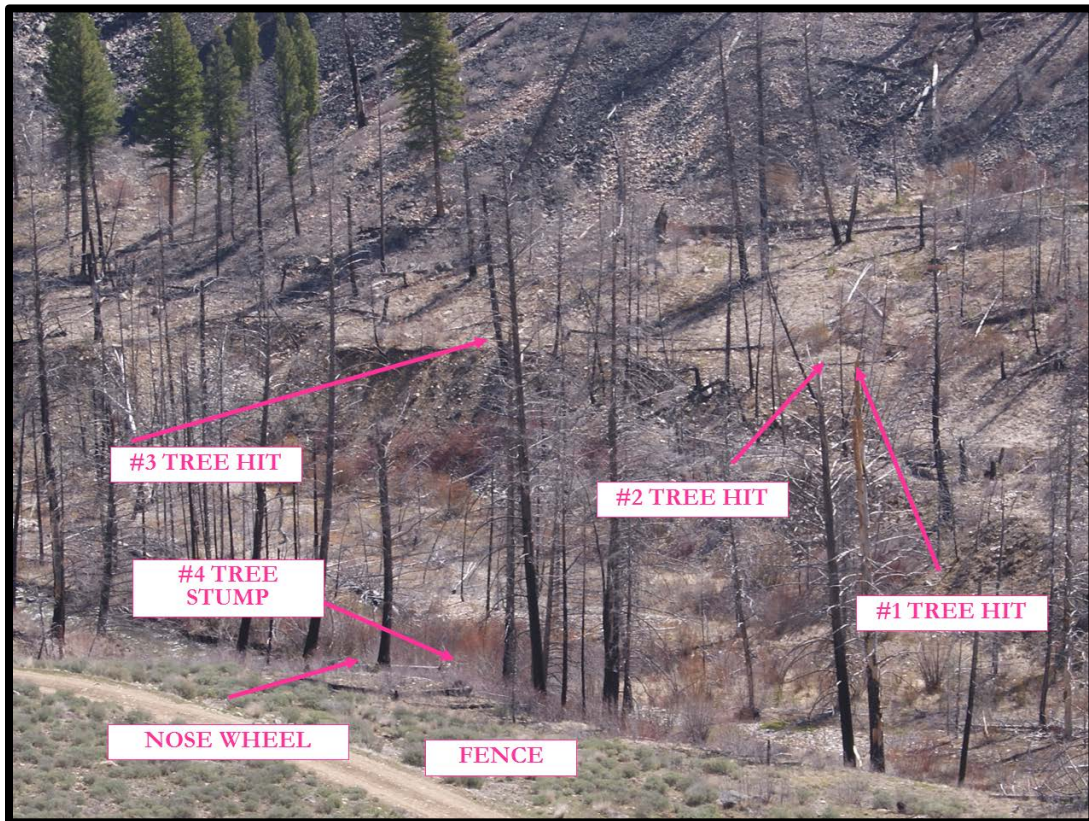
Picture 12: The Trees in Flight Path
