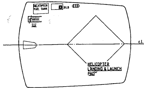
PILOT HOUSE TOP
