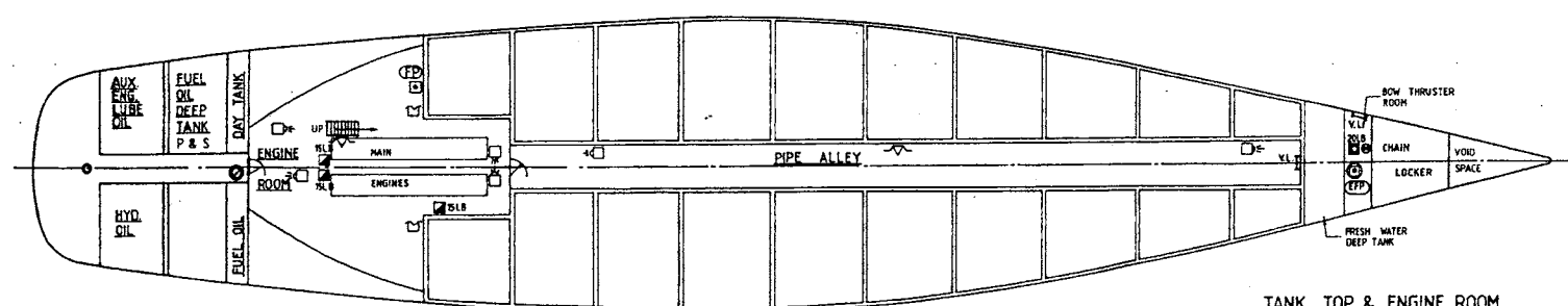
TANK TOP & ENGINE ROOM
