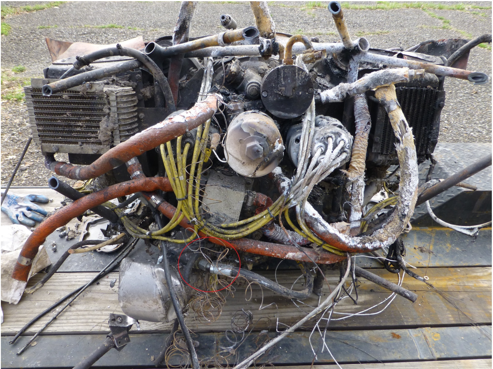
Photo 4 – Rear of engine, loose fuel line in red circle.
