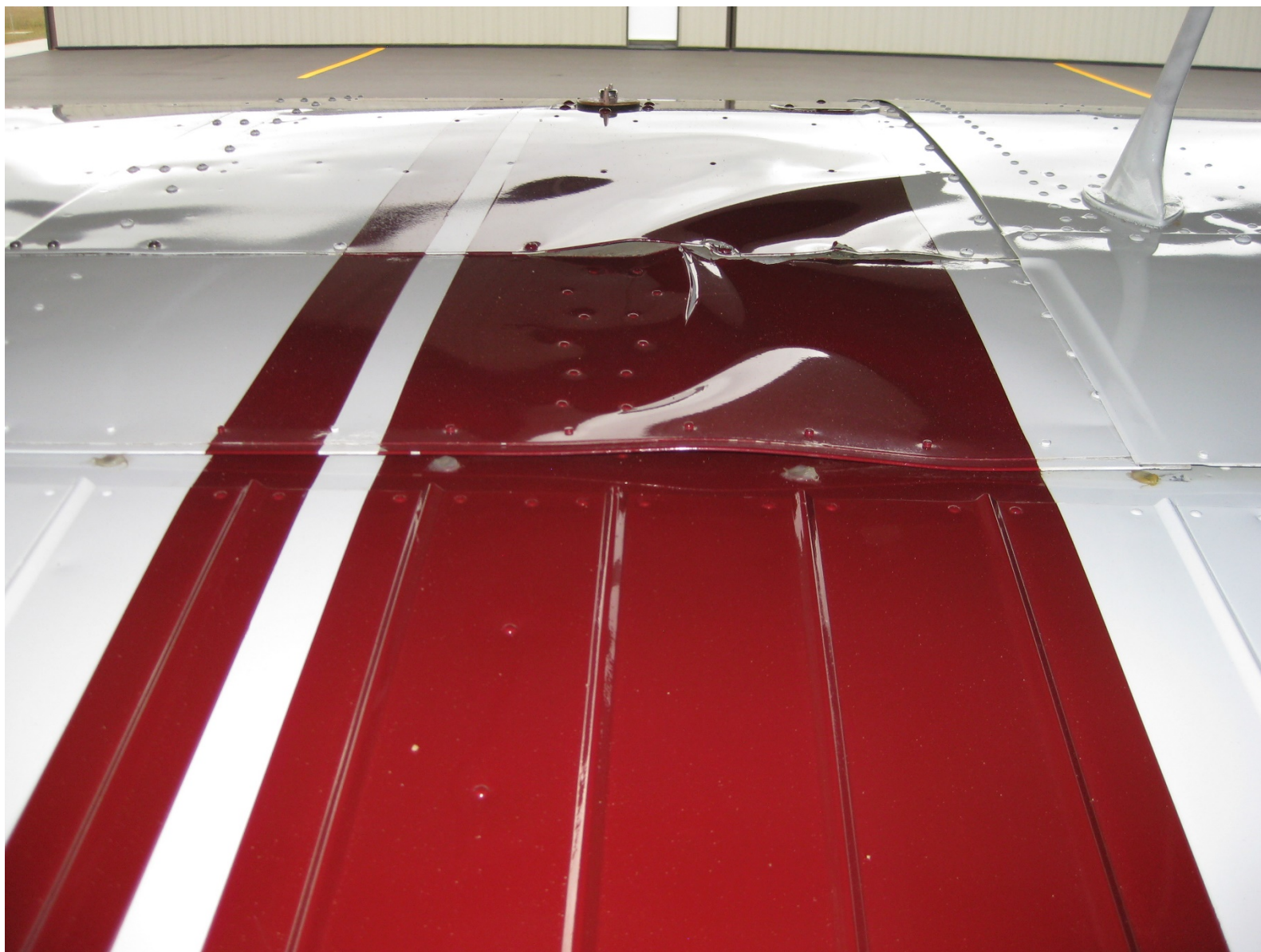
Photo 3 – View of Left Wing Damage (Courtesy of FAA)
