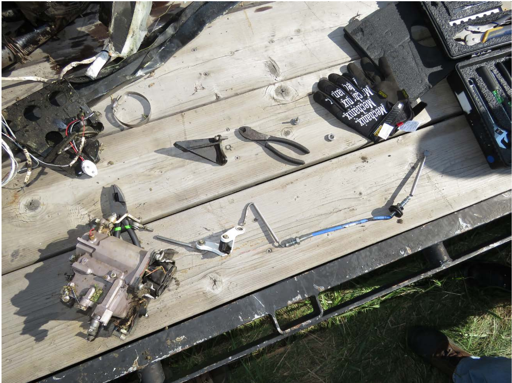
Photo 7 – View of throttle control system after recovery from crash site and wreckage. (Lycoming Engines)
