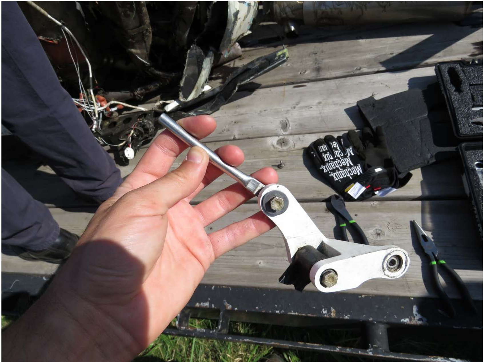
Photo 5 - View of internally-threaded portion of the two-piece throttle control tie rod still attached to the throttle control bellcrank. (Lycoming Engines)
