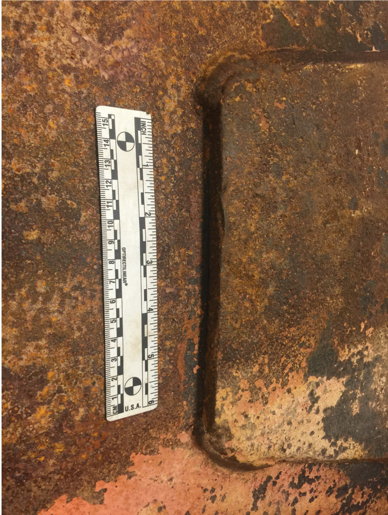
Inboard B-end cradle pad and weld terminations
