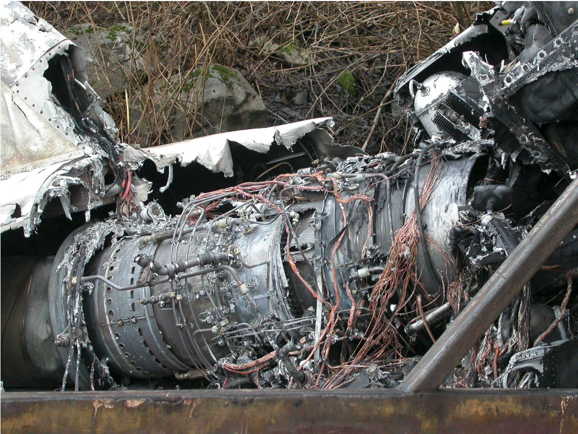
View of fire damage to fuselage and engine along right side of airplane.
